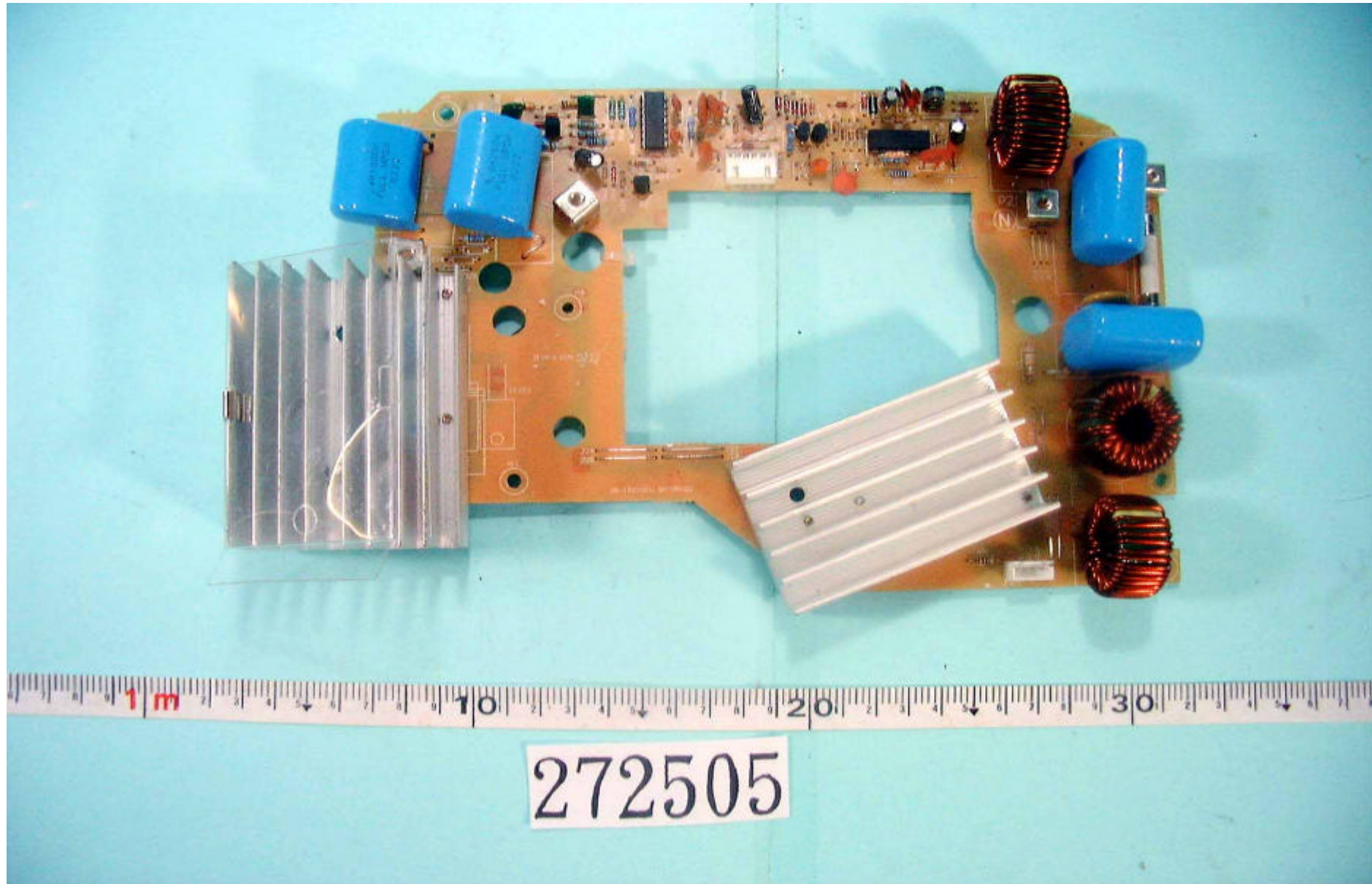
Front SIDE Main board
