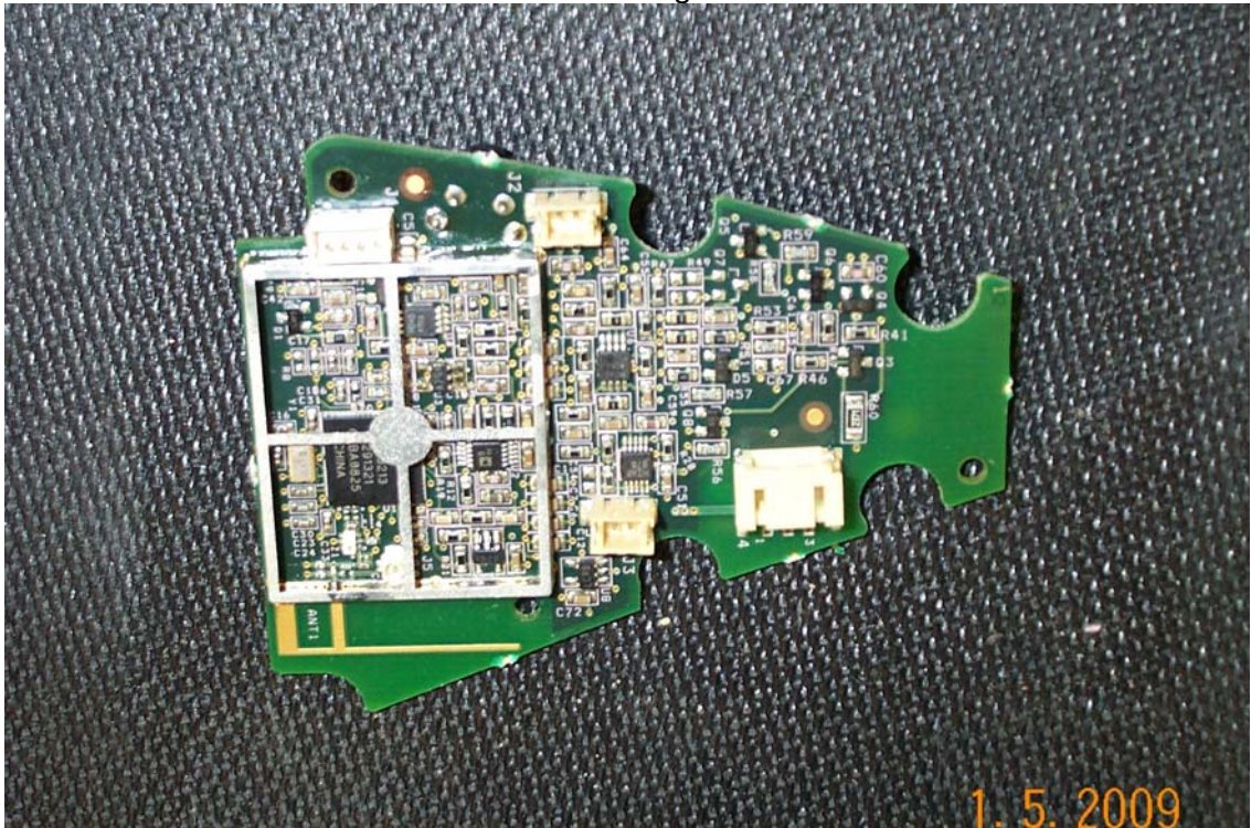
Circuit Board – Cage removed
