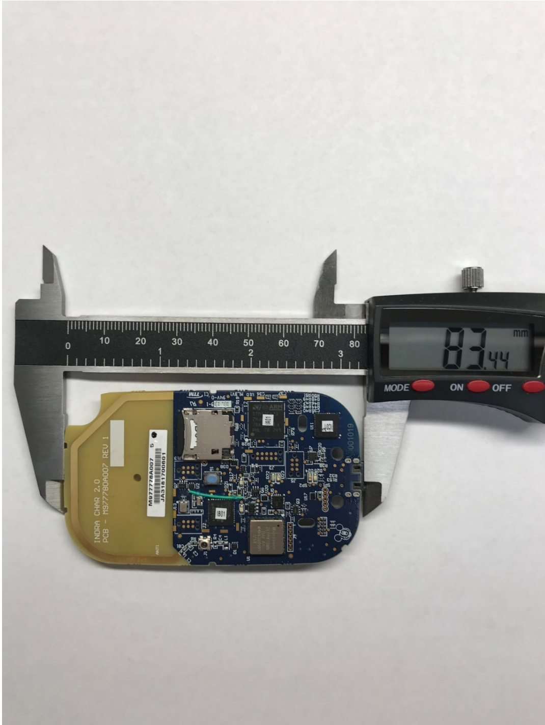
Figure 2: Communicator, Model TM91, Hybrid Front View (Length)
