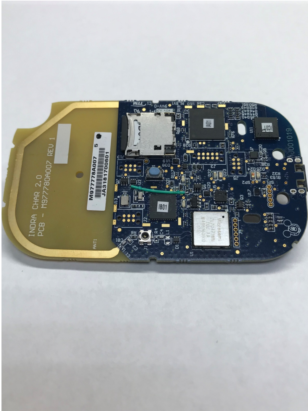
Figure 5: Communicator, Model TM91, Hybrid Left Side View
