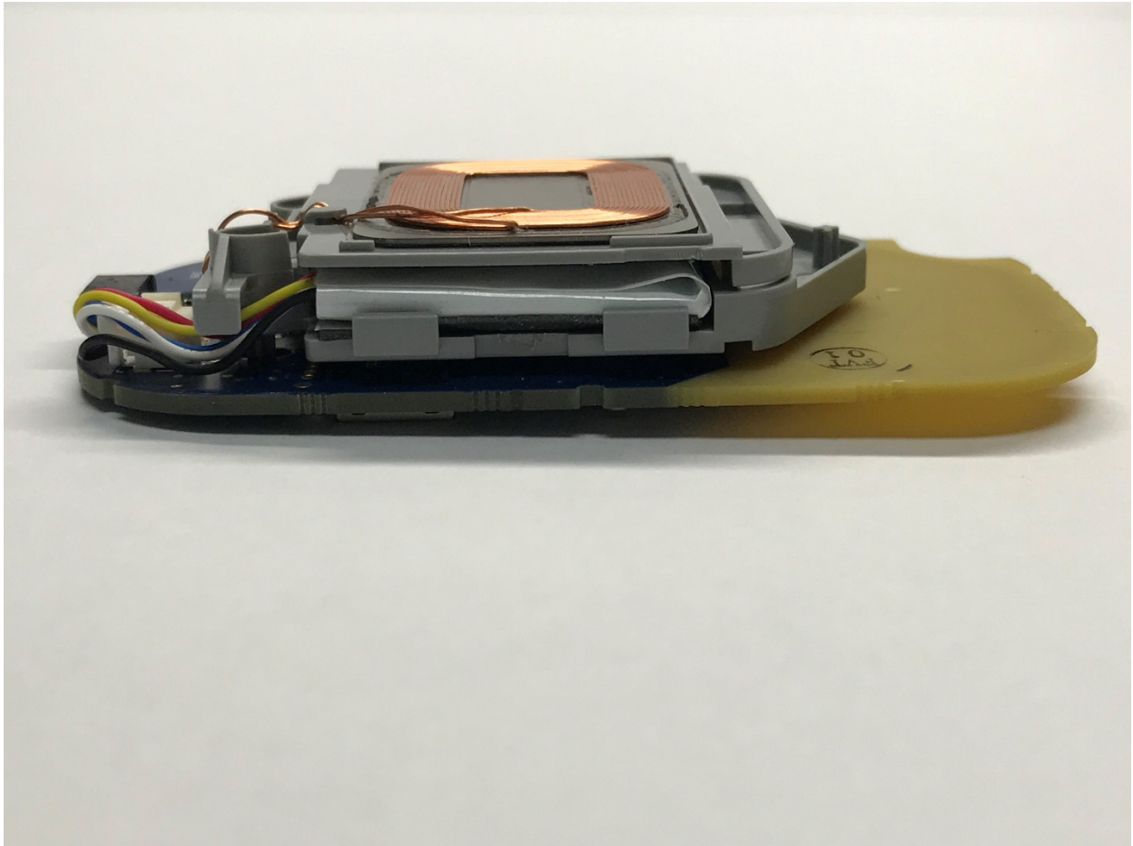
Figure 14: Communicator, Model TM91, Hybrid Inside Housing Side View
