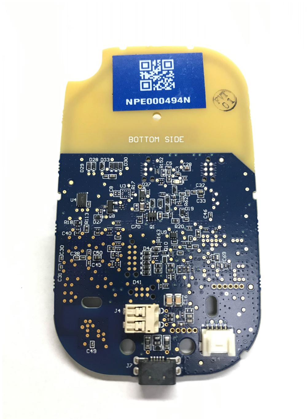
Figure 8: Communicator, Model TM91, Hybrid Bottom Side View
