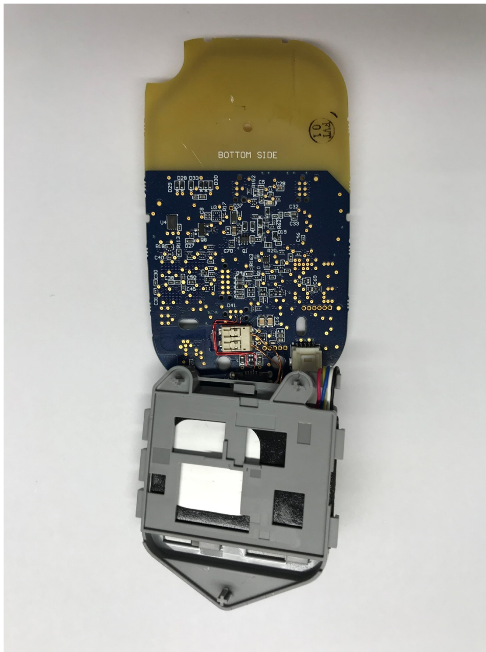
Figure 13: Communicator, Model TM91, Hybrid Inside Housing Flipped View
