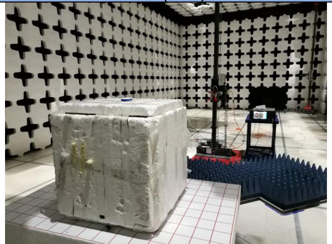
Radiated Emissions (1GHz-6GHz) – Rear View
