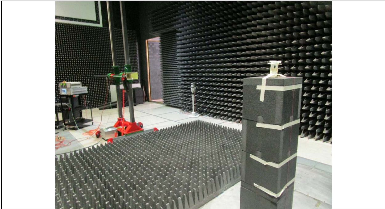
Radiated Emissions Setup Above 1 GHz
