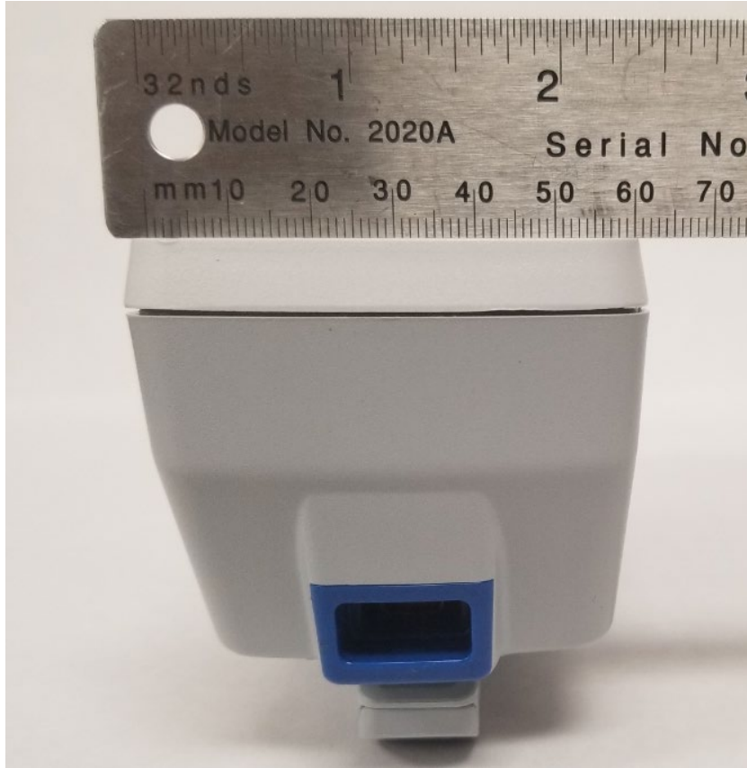
Figure 7 NIM Vital Patient Interface NIM4CPB1 Rear View with dimensions
