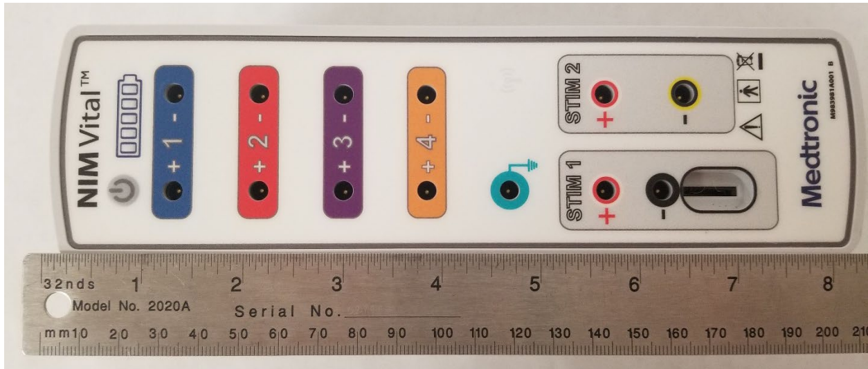
Figure 1 NIM Vital Patient Interface NIM4CPB1 Top View with dimensions
