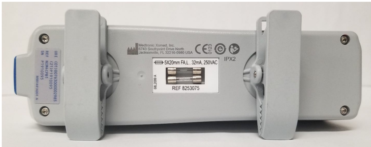
Figure 2 NIM Vital Patient Interface NIM4CPB1 Bottom View
