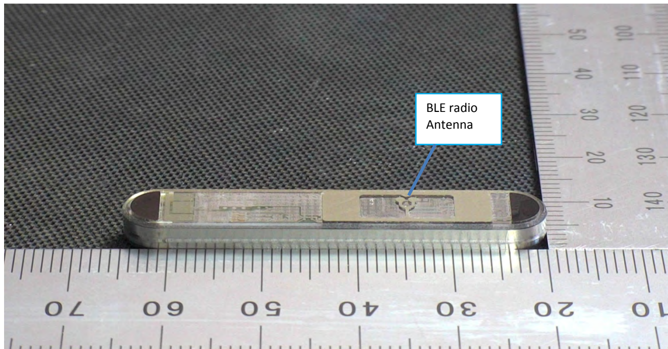
Figure 7 LINQ II Back Top View
