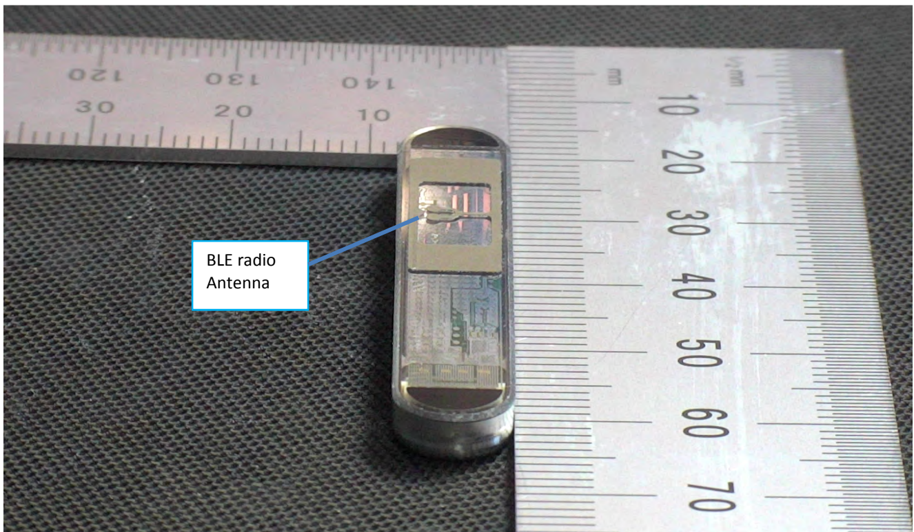
Figure 10 LINQ II Back Right View
