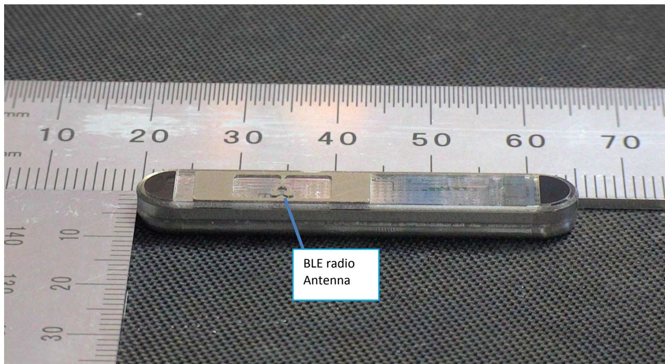
Figure 8 LINQ II Back Bottom View
