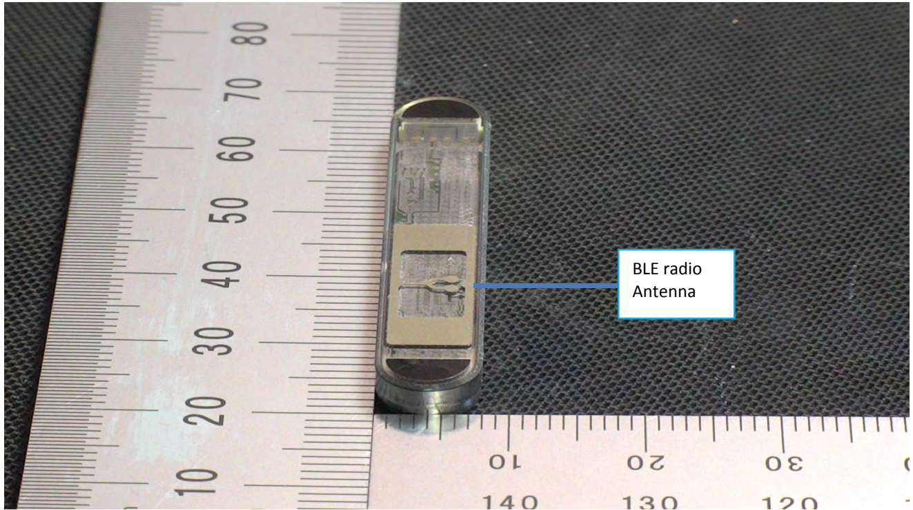
Figure 9 LINQ II Back Left View
