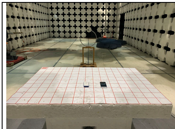
Radiated Emission Test below 30MHz Front View
