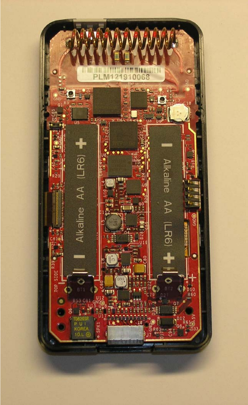
PTM Intellis Model 99745 PCBA Front View
