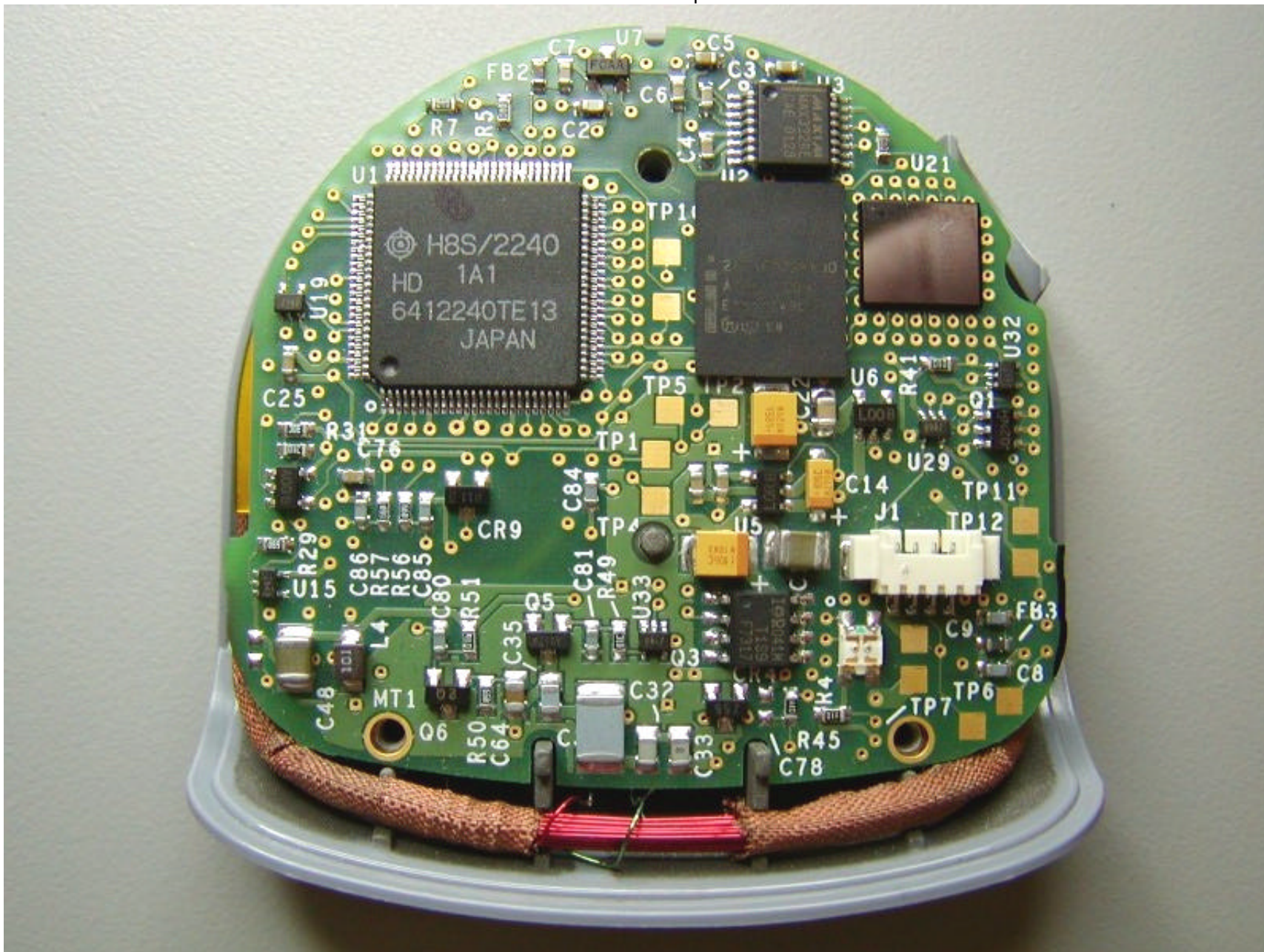
Head PCB Top
