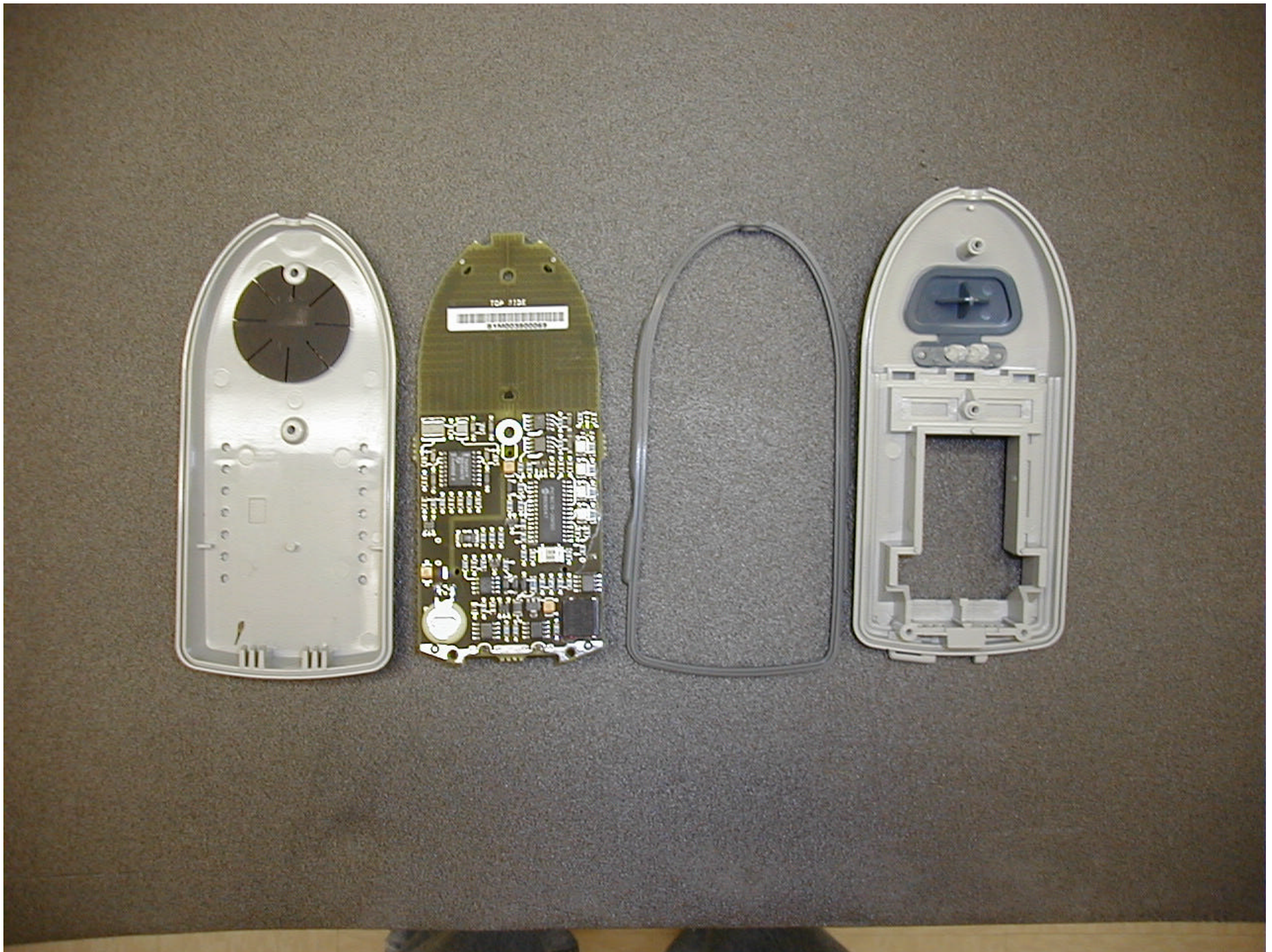
Disassembly – inside view from front
