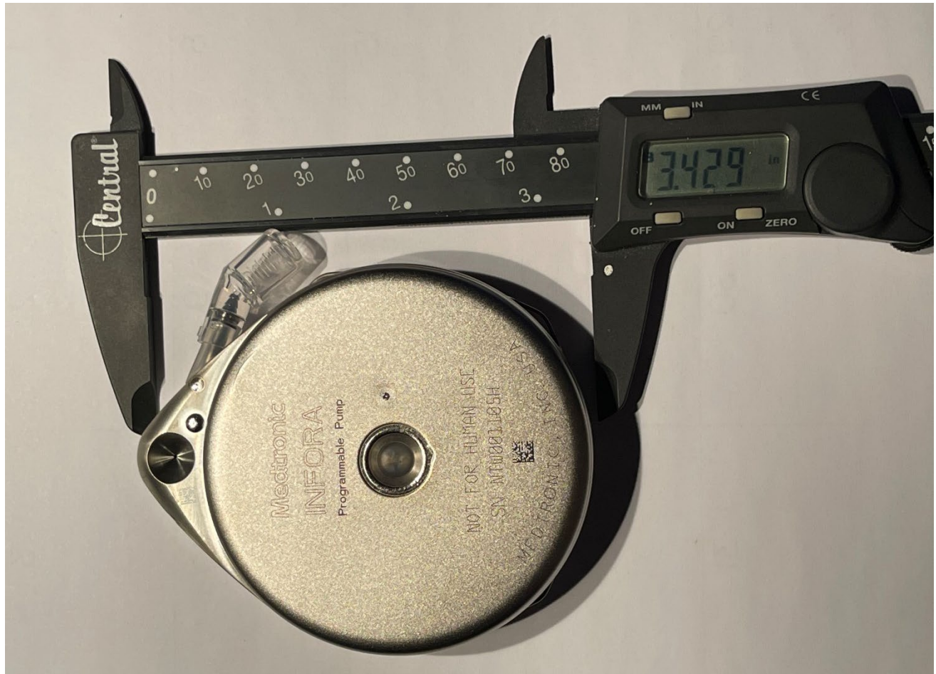
Figure 4: INFORA, Model 8667-20, Side View (Height)
