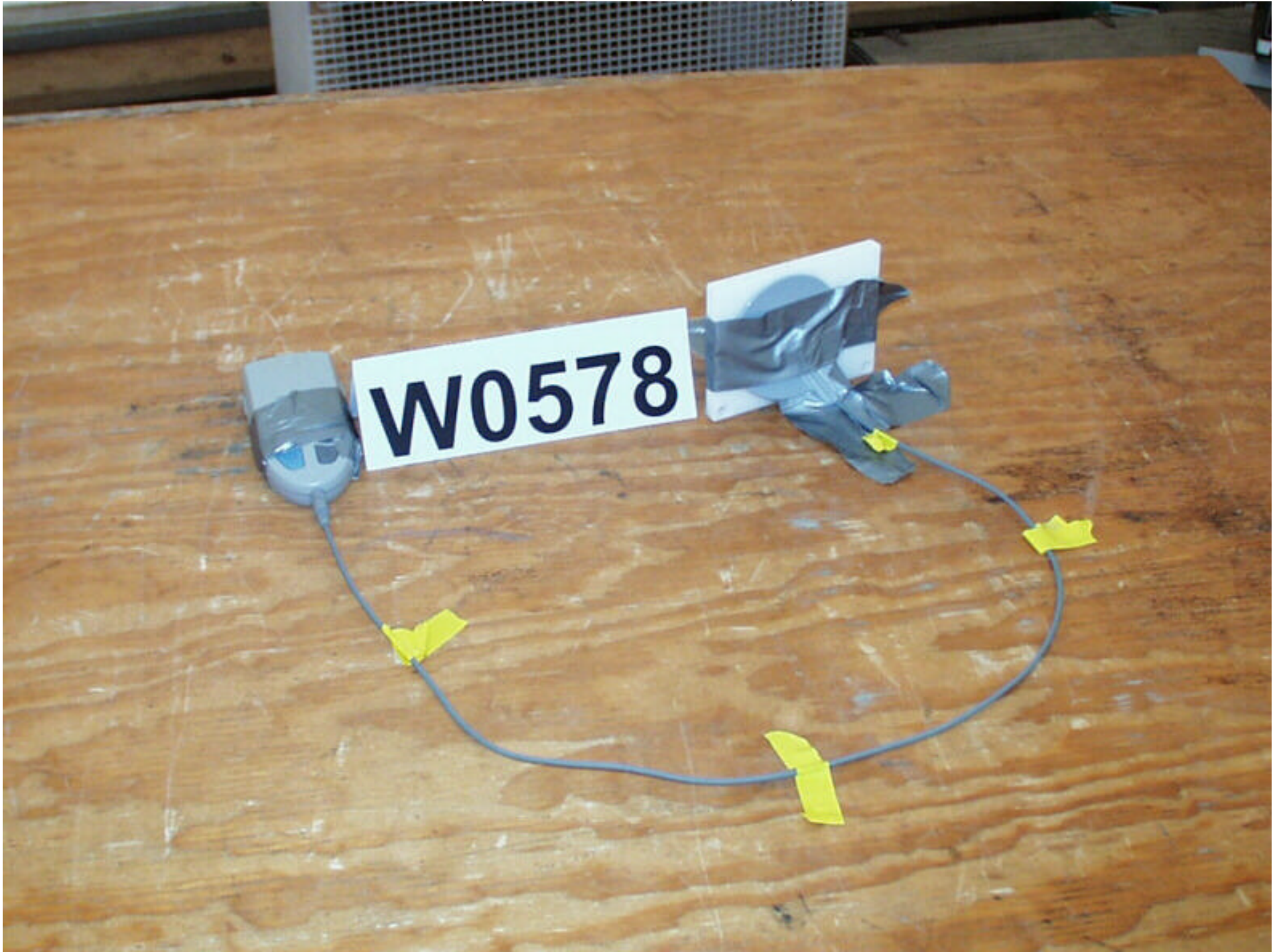
7434A Patient Programmer (representative of Models 3031A and 7438) Radiated Emissions Test Setup (shown with 7440 36" External Antenna)
