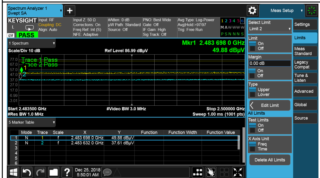
BLE-2480MHz Peak
