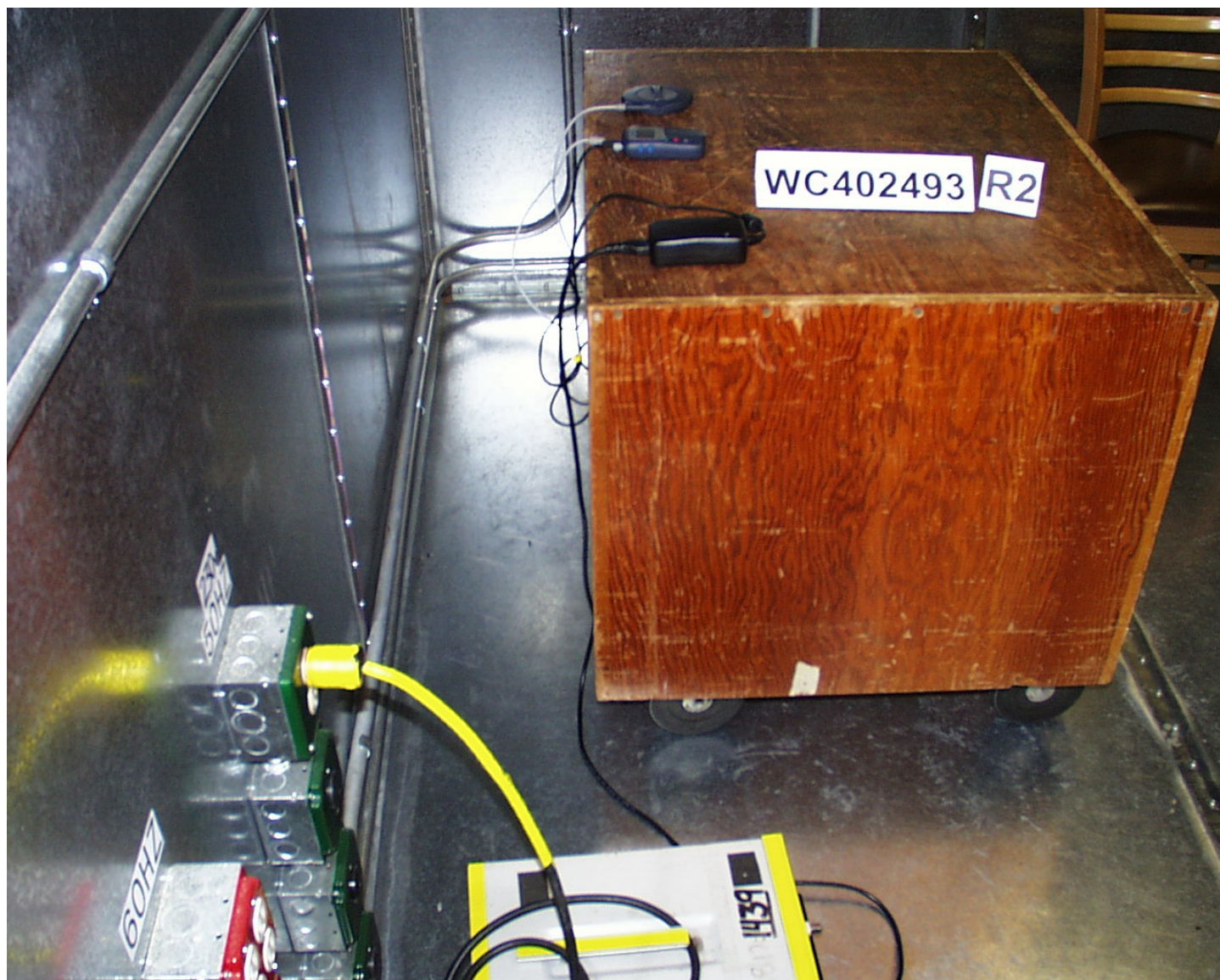
Test-setup photo(s) - (175 kHz): Conducted emission 450 kHz - 30 MHz
