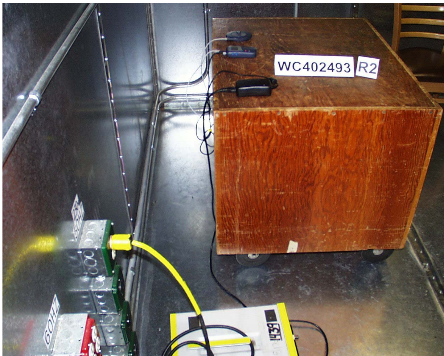
Test-setup photo(s): Conducted emission 450 kHz - 30 MHz
