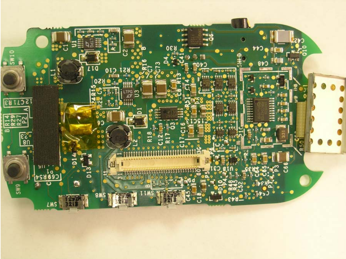
Patient Programmer - Bottom of Board 2
