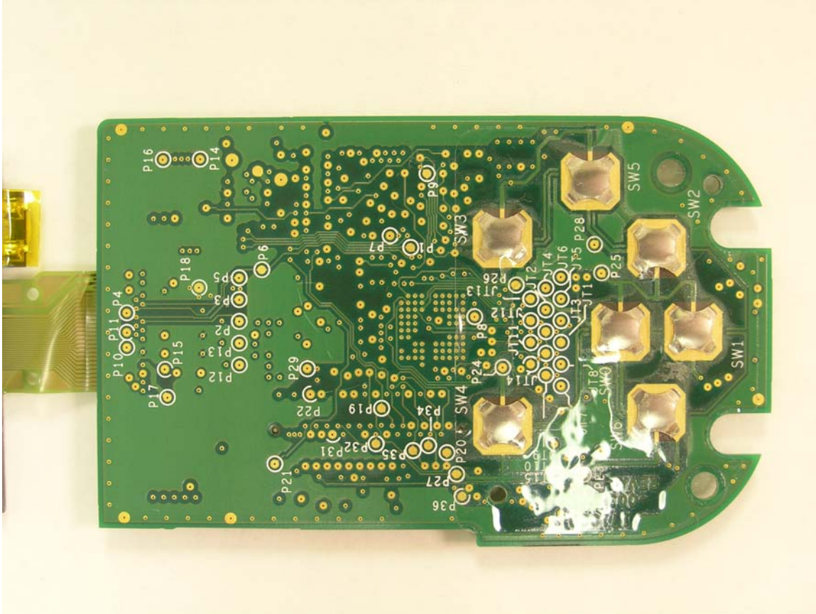
Patient Programmer - Top of Board 2
