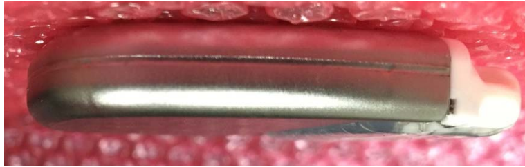
Figure 8: ACTIVA® RC, Model: 37612, Right Side View
