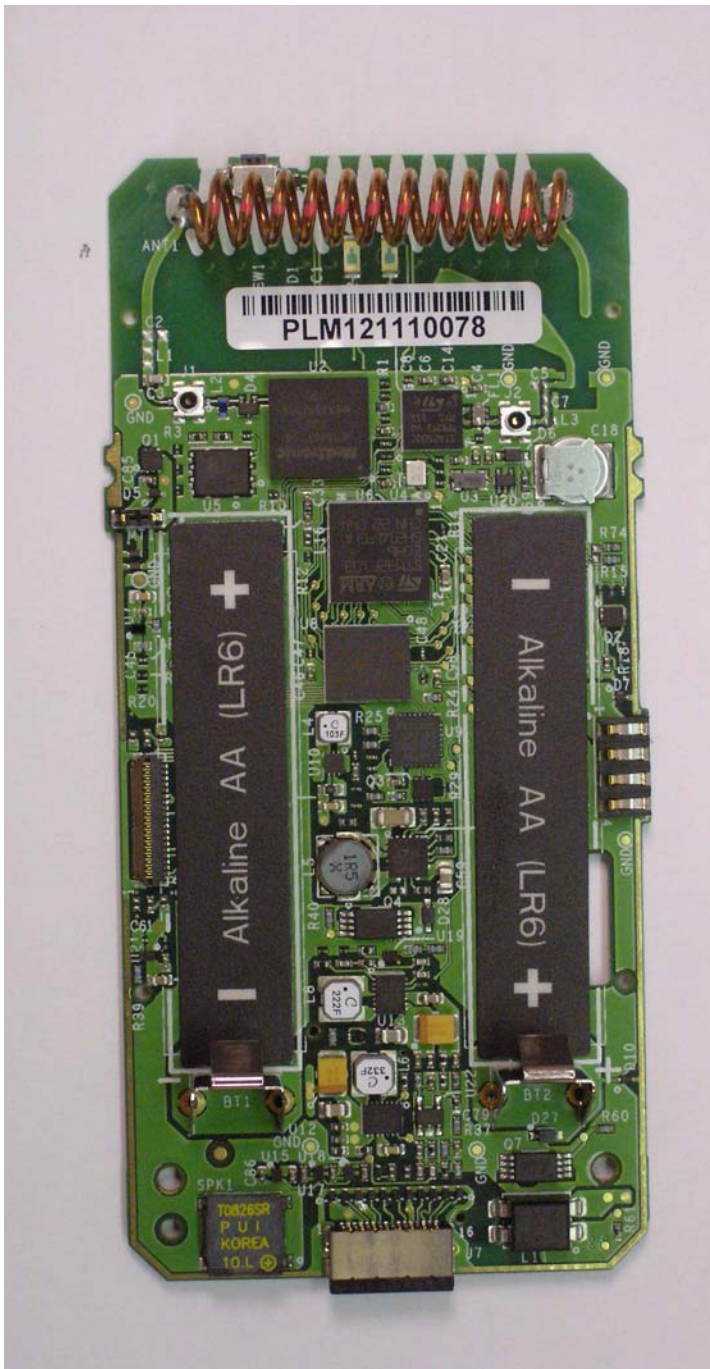
PTM Interstim Model 3537 PCBA Front View
