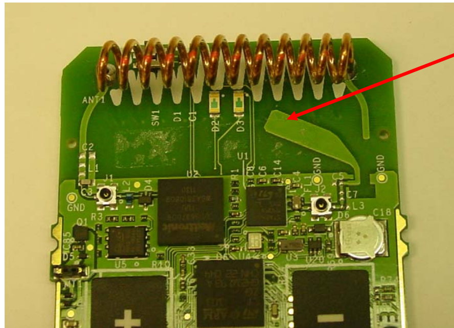
Bluetooth Antenna
