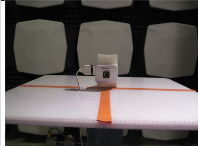
EUT Vertical orientation
