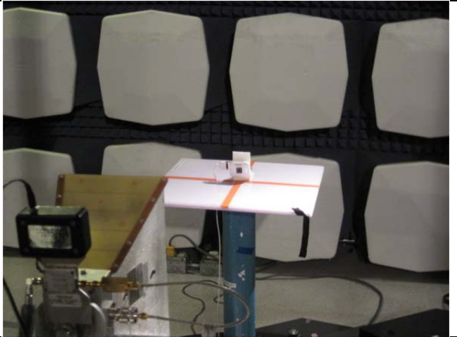
EUT on pedestal
