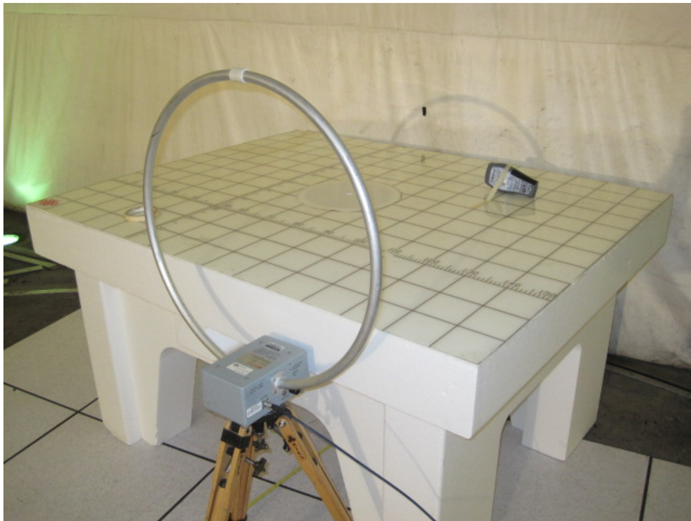
Test-setup photo(s):
