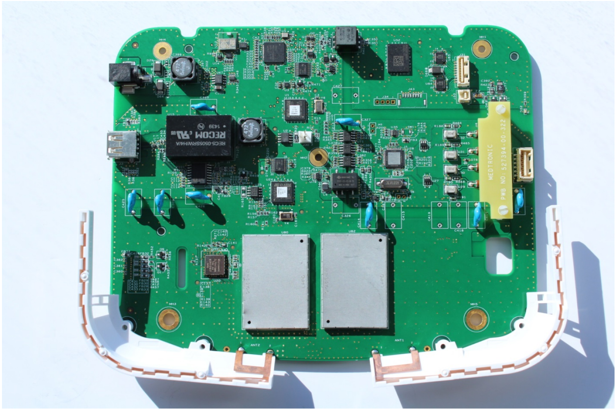
Top View with RF Shields Installed
