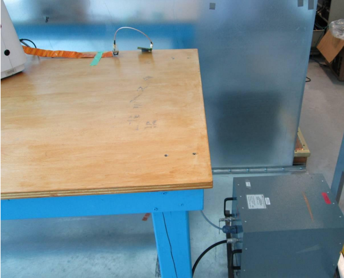
Conducted Emissions
