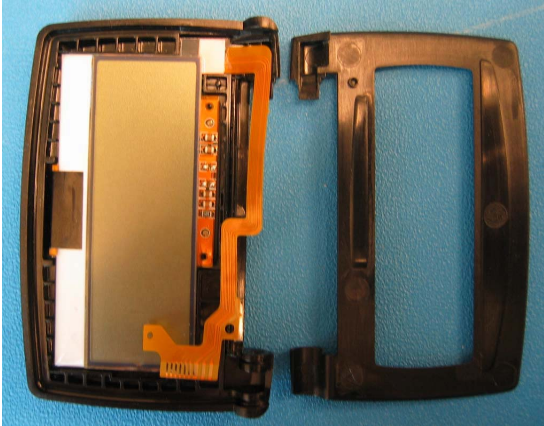
VIEW OF DISPLAY LID – INTERNAL
