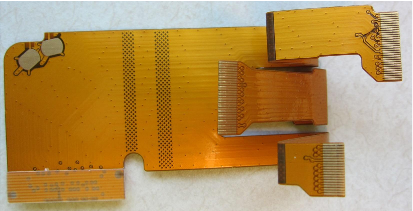
Figure 18: Keyboard interconnect FPC top
