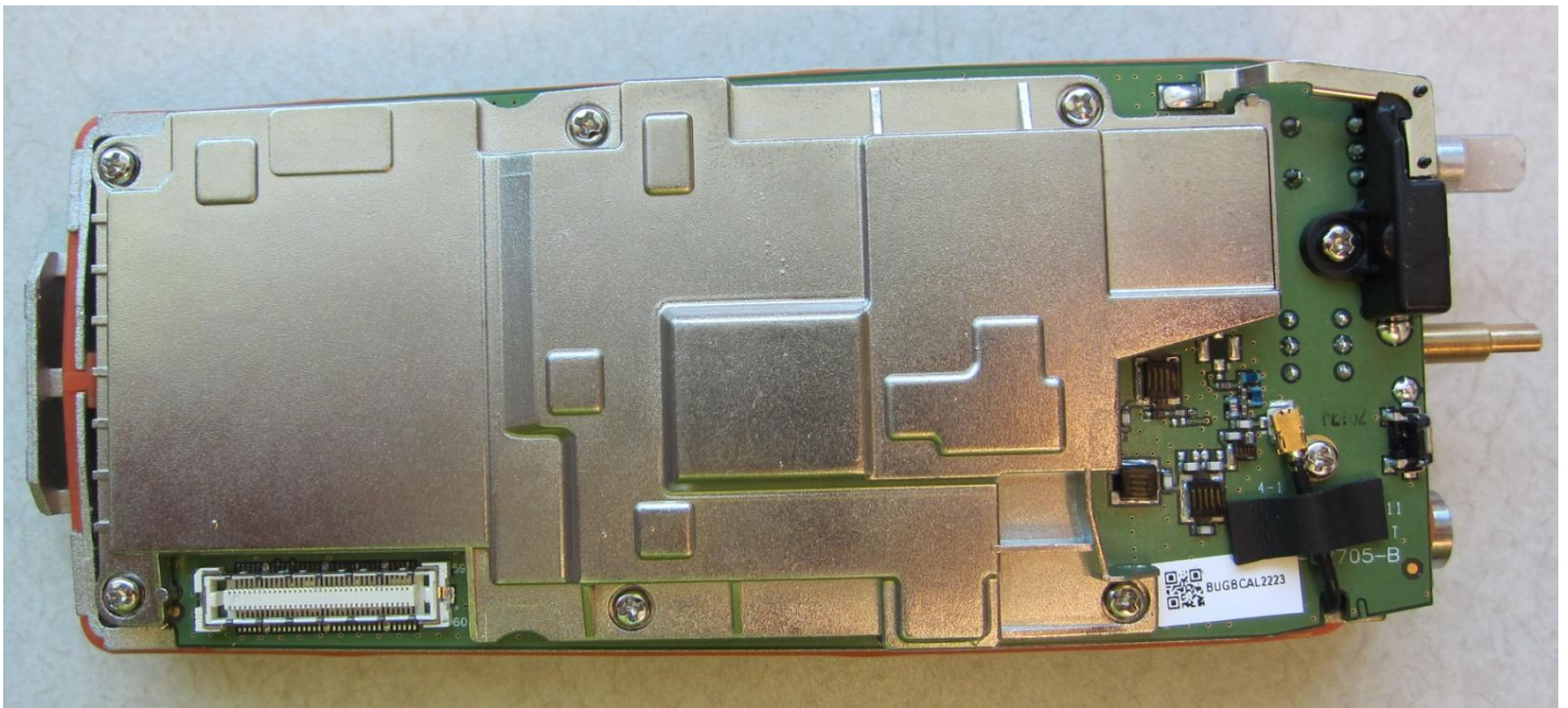
Figure 3: Main PCB assembly - bottom view
