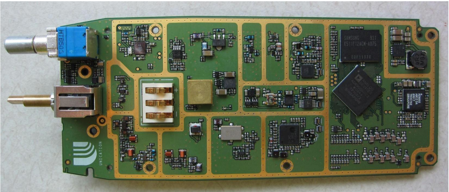
Figure 6: Main PCB - bottom side
