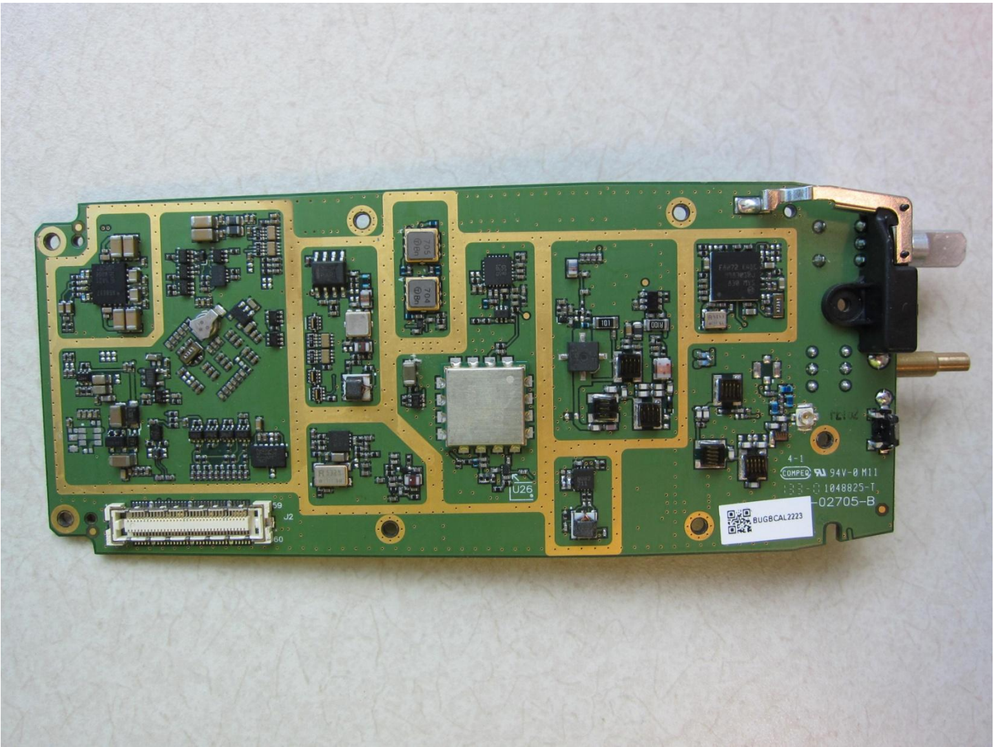
Figure 5: Main PCB - top side
