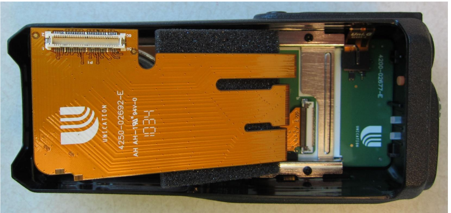
Figure 2: U3 Internals with main PCB removed - right side
