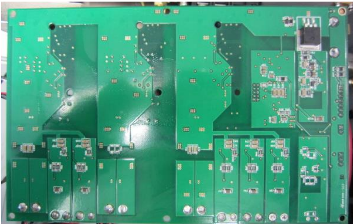
Figure 24 TX_PSU_PCB Bottom View
