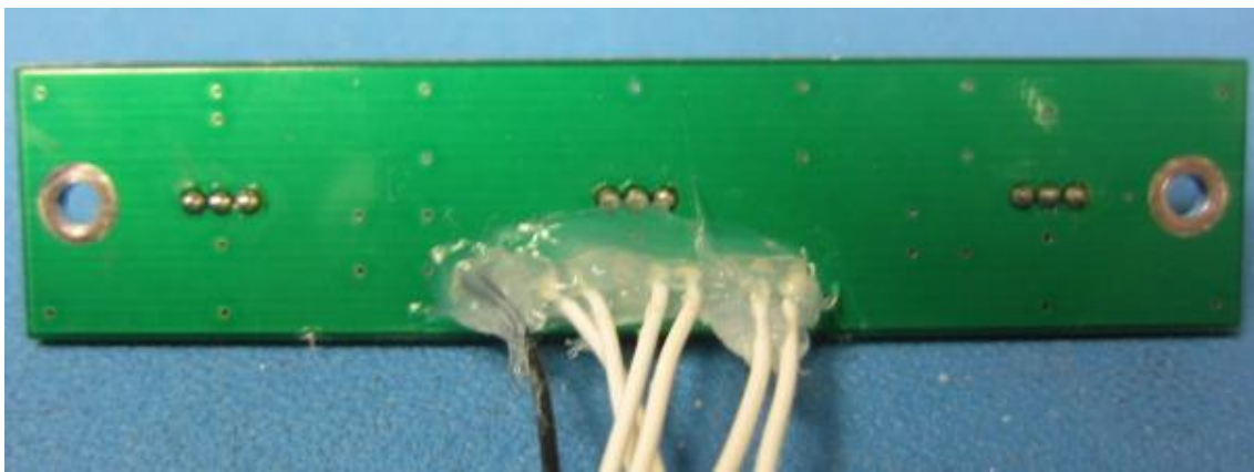
Figure 28 TX_LED_PCB Bottom View
