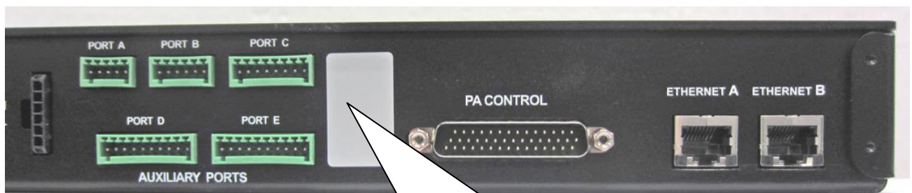
Figure 4: R01 VHF Receiver Rear Panel
