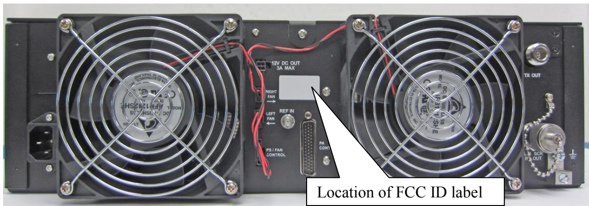
Figure 2: R01 VHF Transmitter Rear Panel
