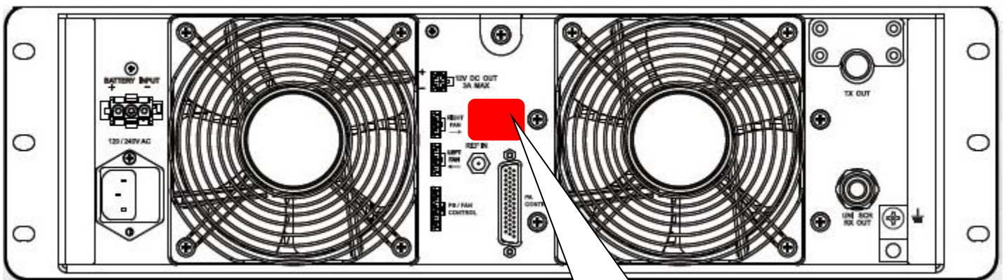
Figure 2: R01 7/800MHz Transmitter Rear Panel
