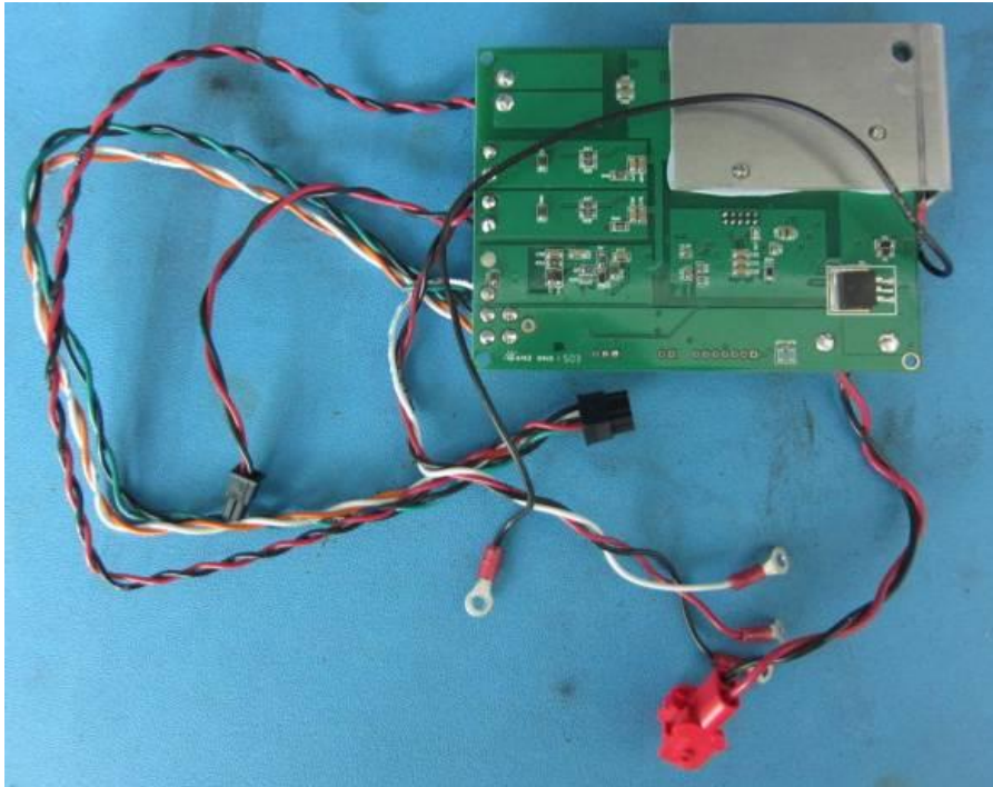
Figure 3: RX PSU PCB with Cables
