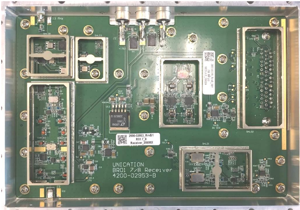
Figure 15: RX 700/800MHz Receiver PCB Top View (Shield covers removed)
