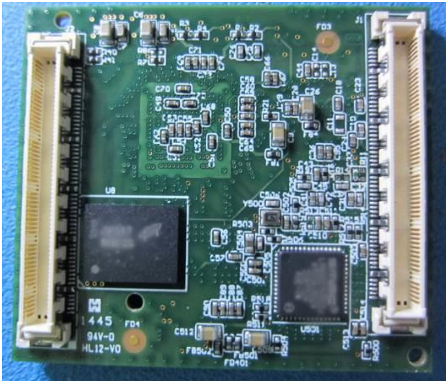
Figure 20: RX CPUM PCB Bottom View
