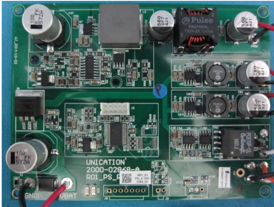
Figure 1: RX PSU PCB Top View
