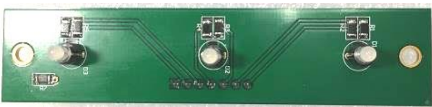
Figure 35: TX LED PCB Top View
