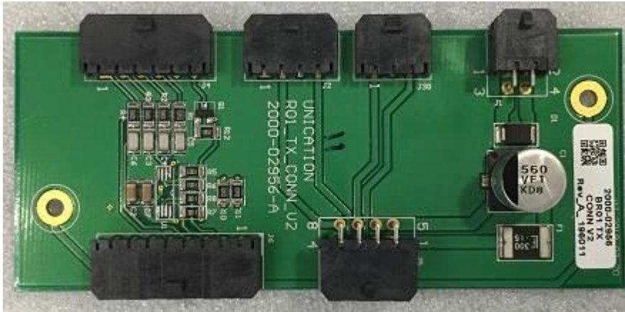
Figure 33: TX Fan PCB Top View
