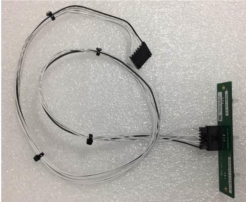
Figure 37: TX LED PCB with Cable
