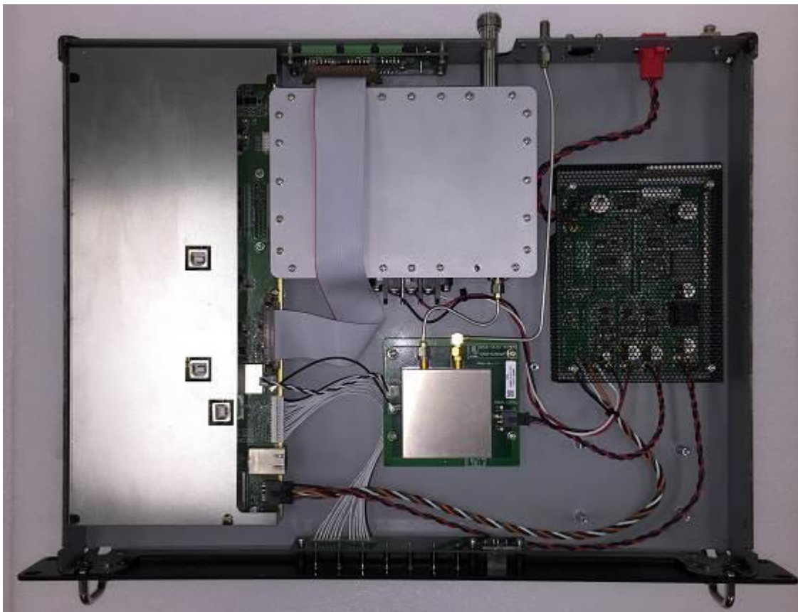
Figure 24: RX Chassis Top View
