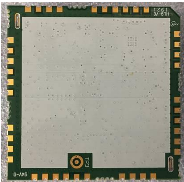
Figure 48: 700/800MHz Local Oscillator PCB Bottom View
