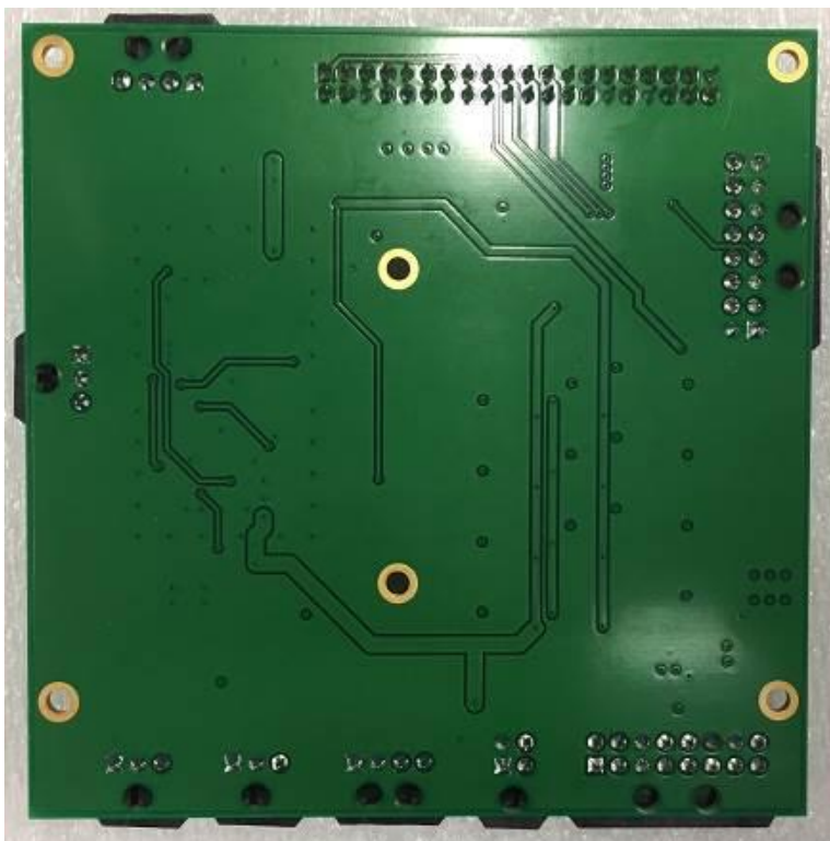
Figure 59: PS Controller PCBA Bottom View
