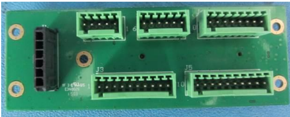
Figure 14: RX AUX V2 PCB Bottom View
