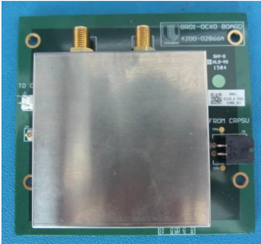
Figure 10: RX OCXO PCB with Shield
