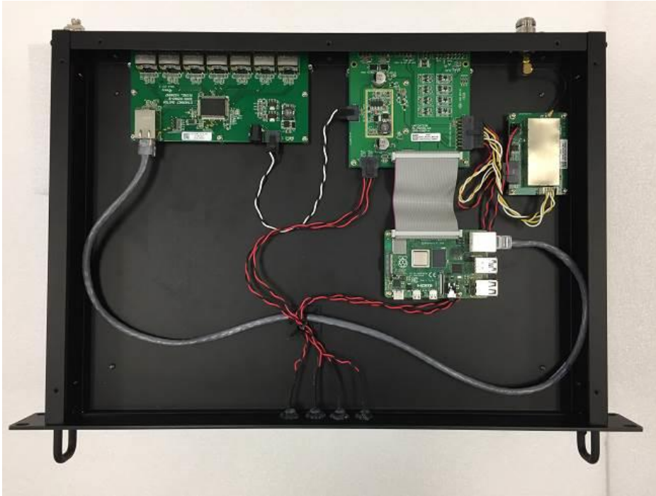
Figure 65: TC01 Trunking Controller Chassis Assembly Top View
