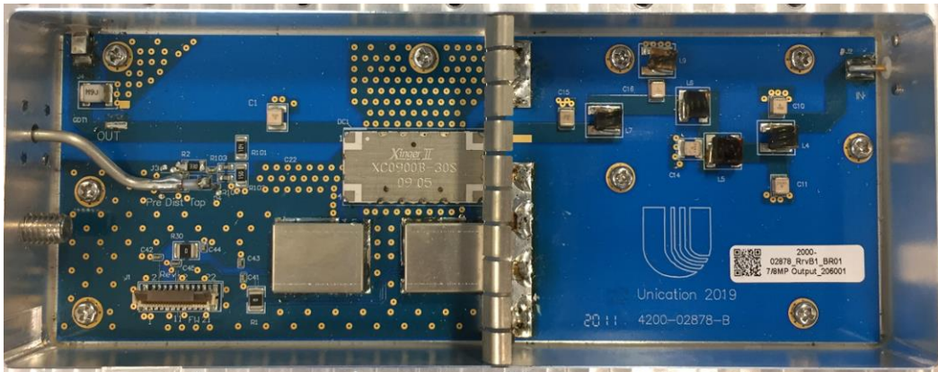
Figure 42: TX 700/800MHz Output Filter PCB Top View
