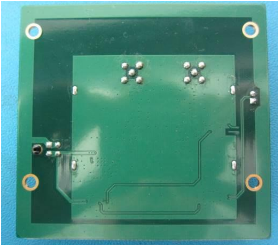
Figure 9: RX OCXO PCB Bottom View
