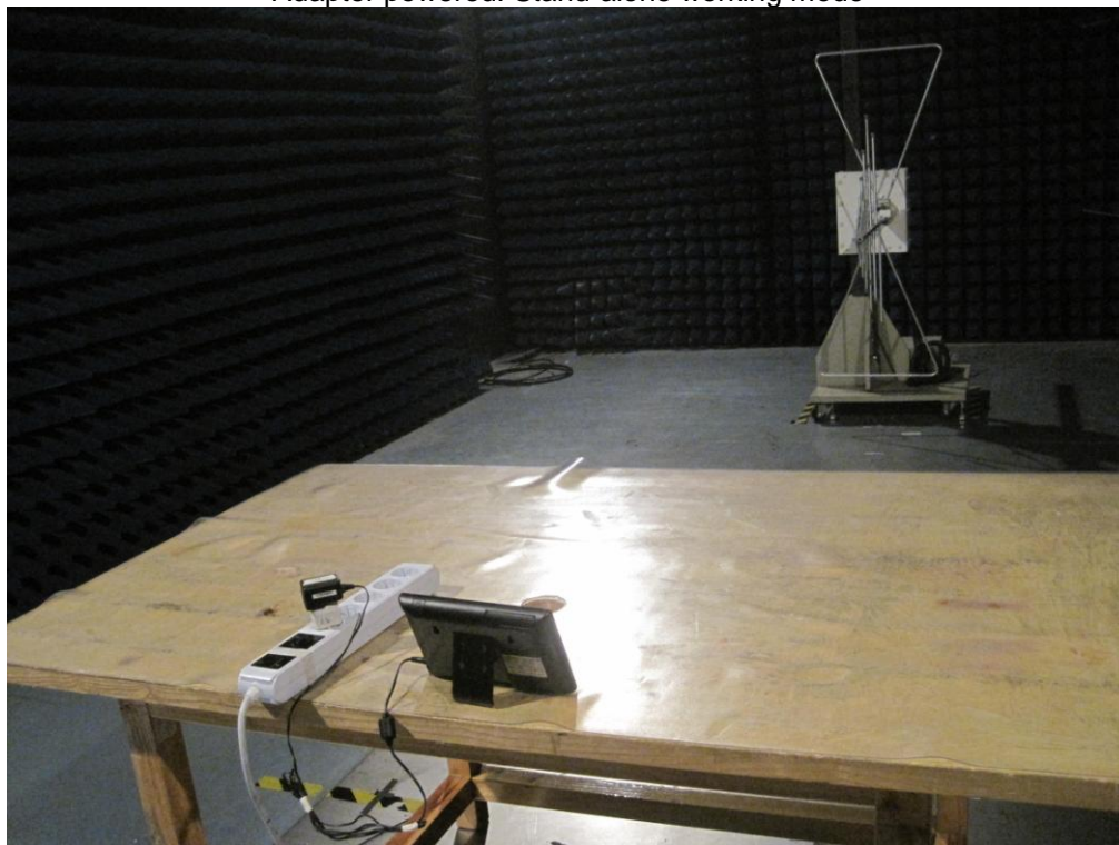
Adapter powered: Stand-alone working mode
