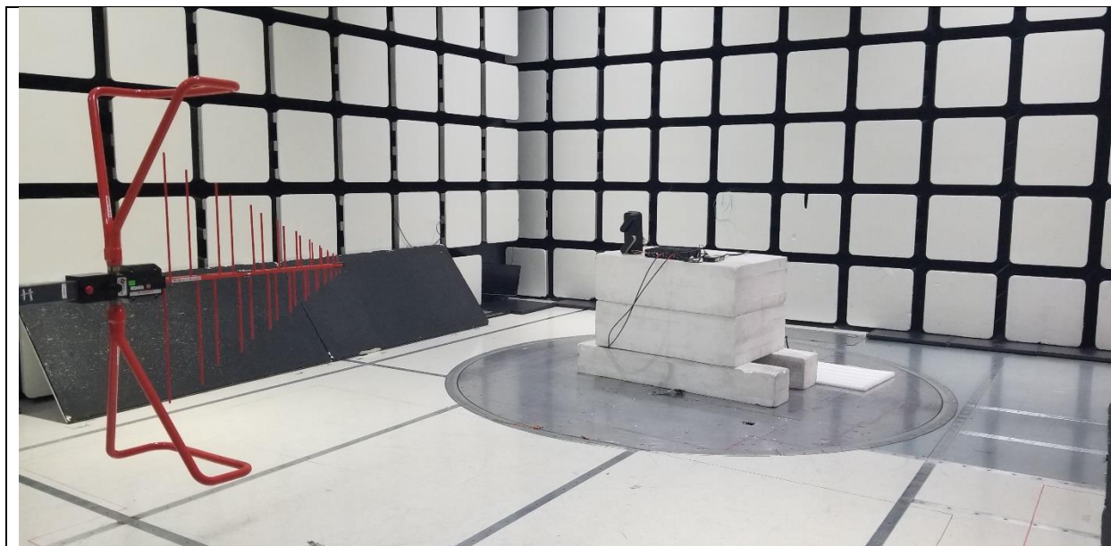
Title: Radiated Spurious Emissions Test Configuration 30M - 1000MHz
