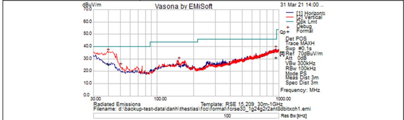
Title: TX Spurious Emissions from 30MHz-1GHz – Ch1 (2412 MHz)
