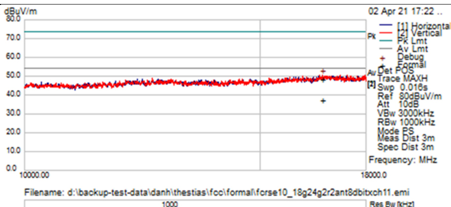
TX Spurious Emissions from 10GHz-18GHz – Ch11 (2462 MHz)
