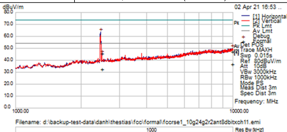
TX Spurious Emissions from 1GHz-10GHz – Ch11 (2462 MHz)
