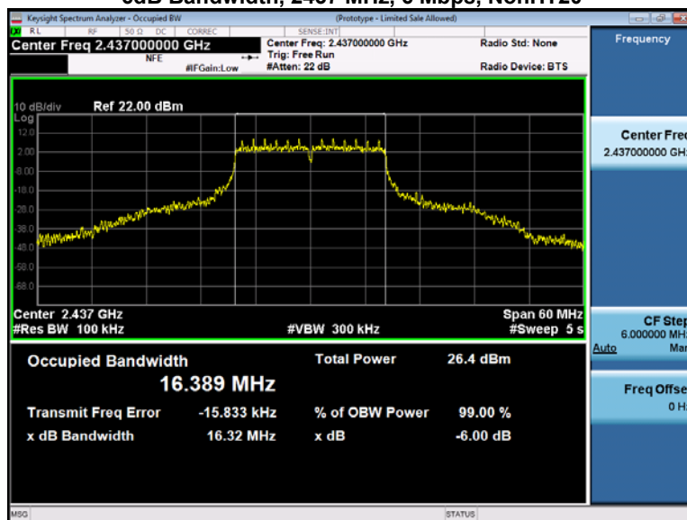
6dB Bandwidth, 2437 MHz, 6 Mbps, NonHT20
