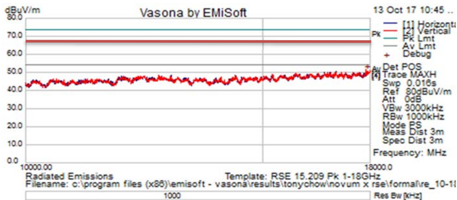
Title: TX Spurious Emissions from 10-18GHz – Ch44 (5220 MHz) – Peak Trace
