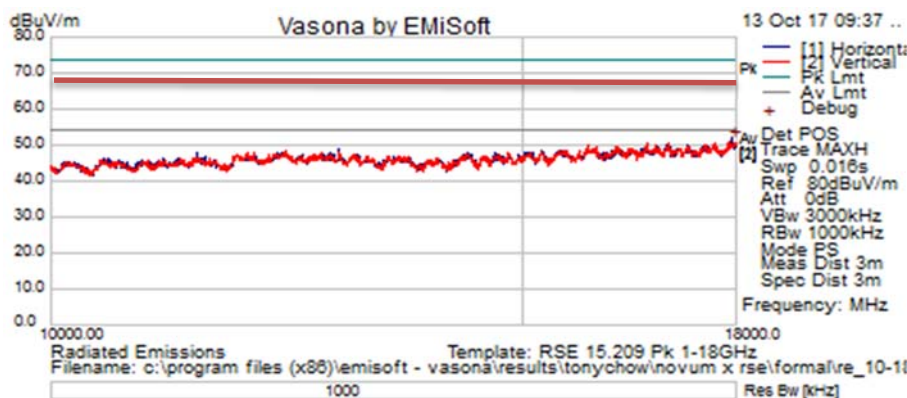
Title: TX Spurious Emissions from 10-18GHz – Ch36 (5180 MHz) – Peak Trace
