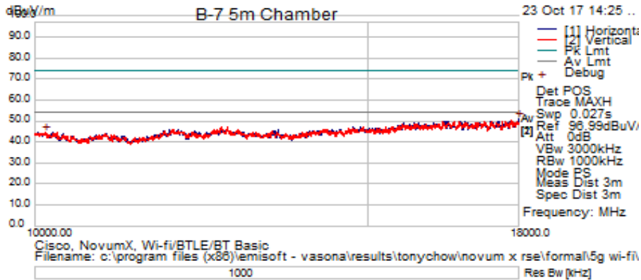
Title: TX Spurious Emissions from 10-18GHz – Ch1 (2412 MHz) – Peak Trace
