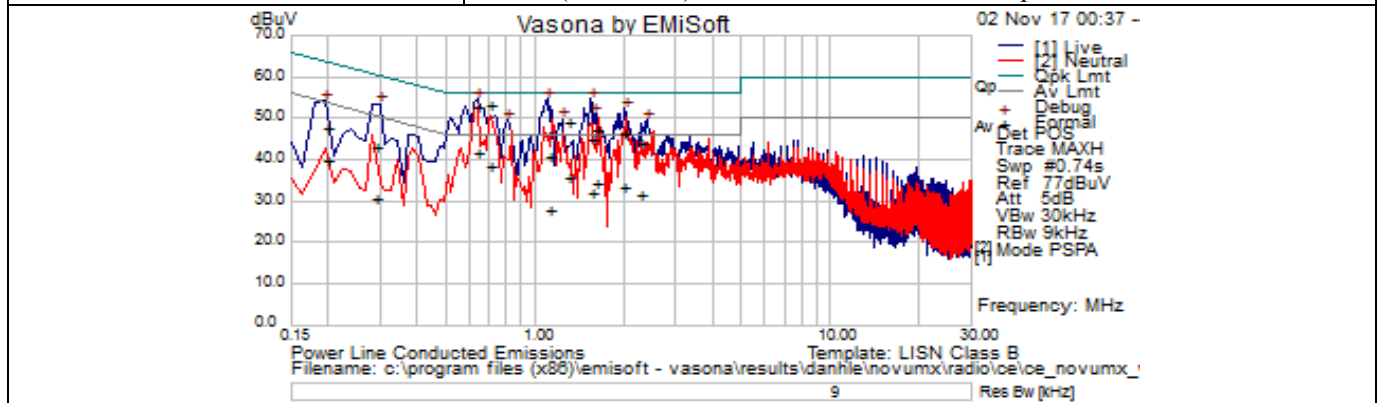
AC Conducted Emissions Test Result Tables for 802.11b / TX Ch6
