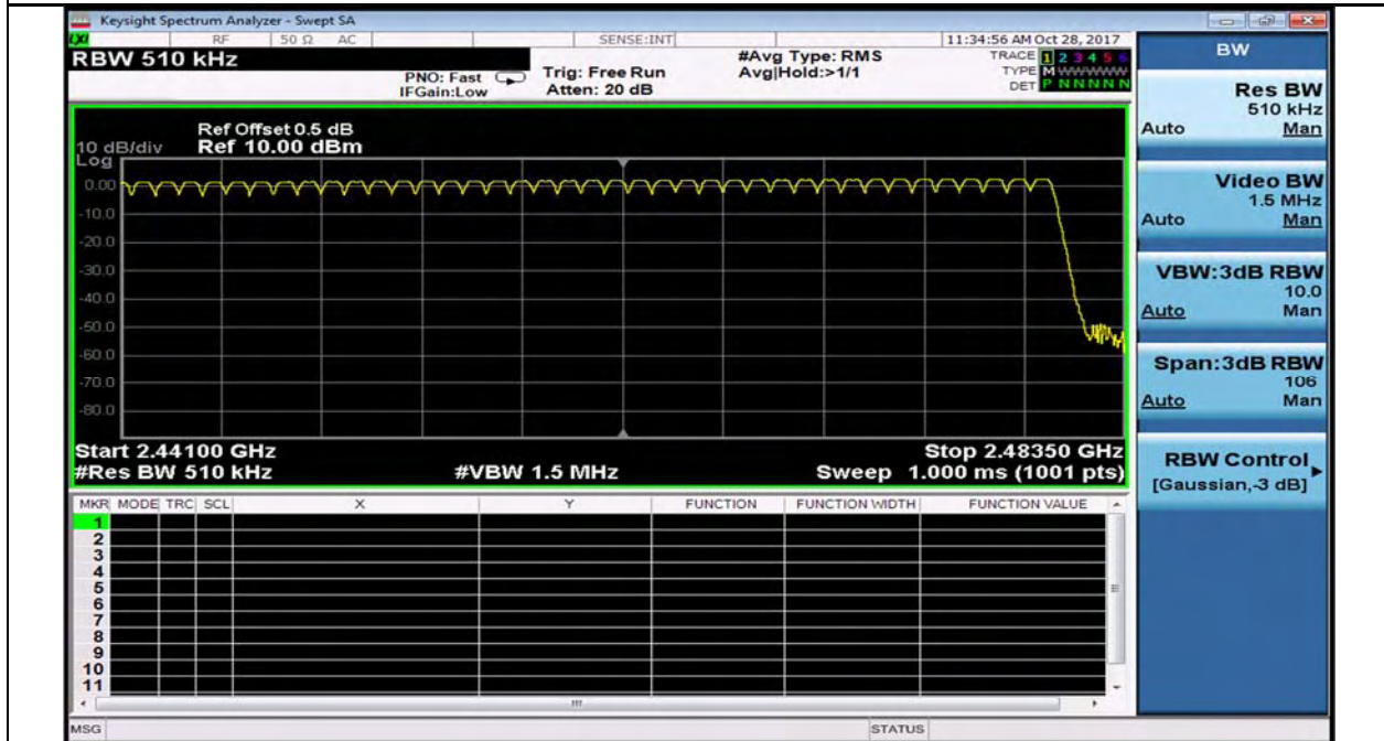
Title: Total No. of Hops Channels = 39.5 for 2 nd segment in the frequency range 2441-2483.5MHz
