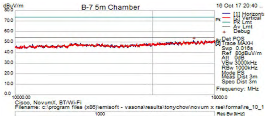
Title: TX Spurious Emissions from 10-18GHz – Ch0 (2402 MHz)
