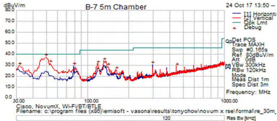
Title: TX Spurious Emissions from 30MHz-1GHz – Ch39 (2441 MHz)
