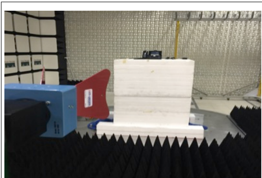
Title: Radiated Emissions Above 1 GHz
