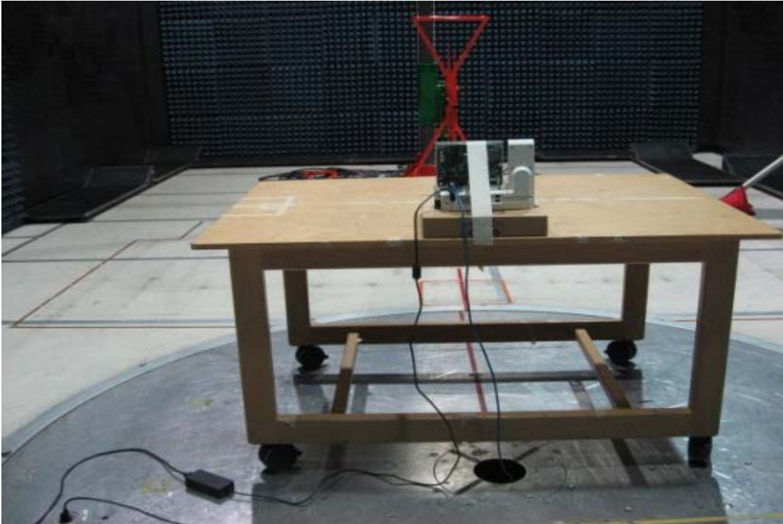
Radiated Emissions Setup Photo: 30-1GHz
