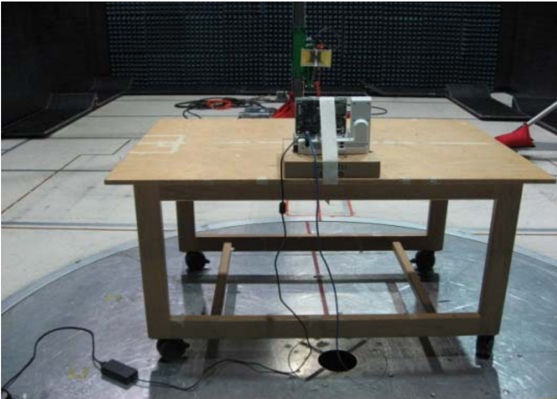
Radiated Emissions Setup Photo: 1-18GHz
