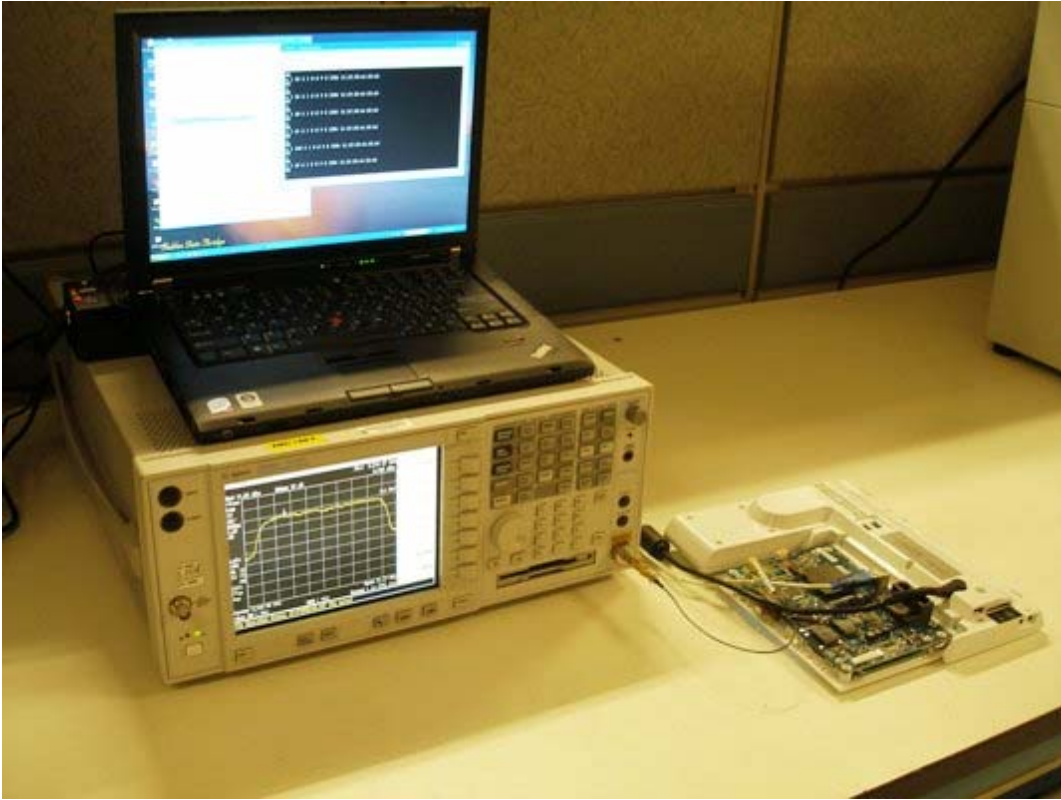
Setup Photo for WiFi Conductive Measurements
