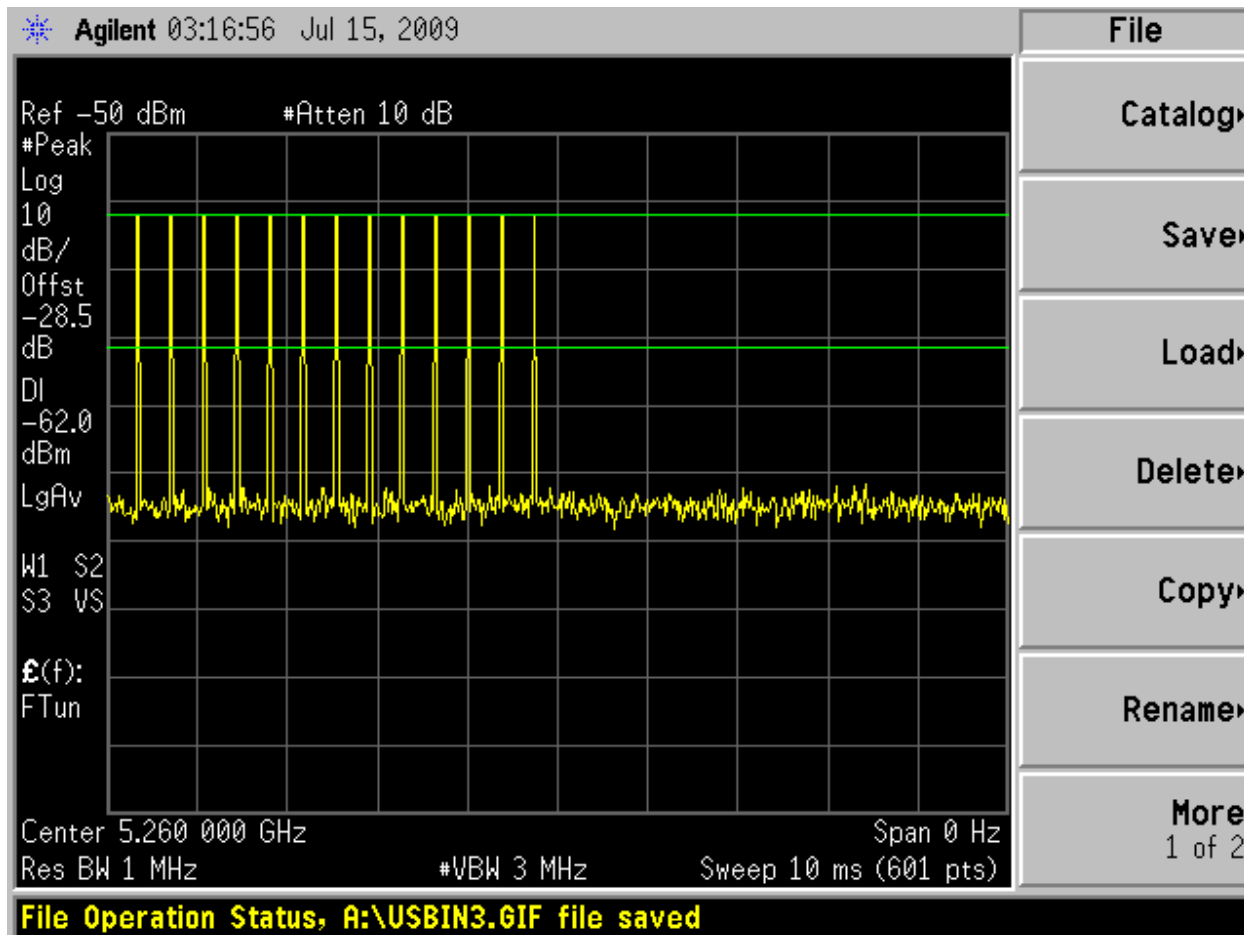
Bin 4 Radar Calibration
