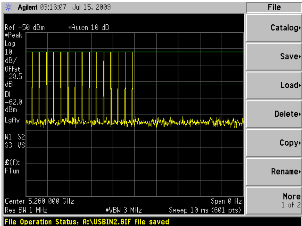
Bin 3 Radar Calibration
