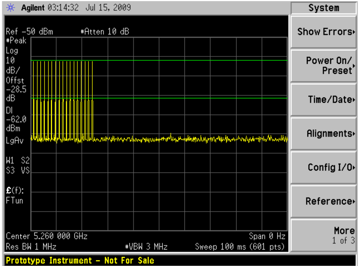
Bin 1 Radar Calibration
