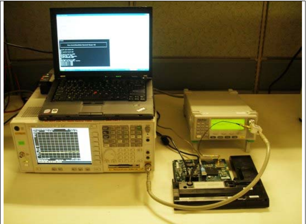
Title: Test setup for all Conducted Emissions testing
