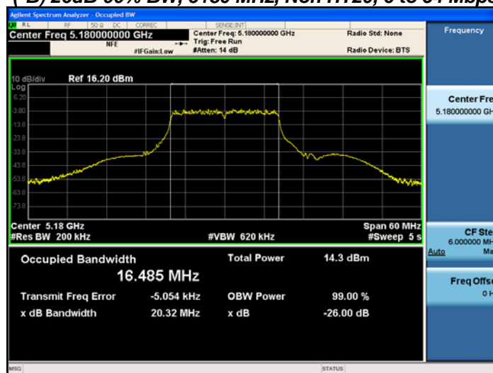
(-B) 26dB-99% BW, 5180 MHz, Non HT20, 6 to 54 Mbps
