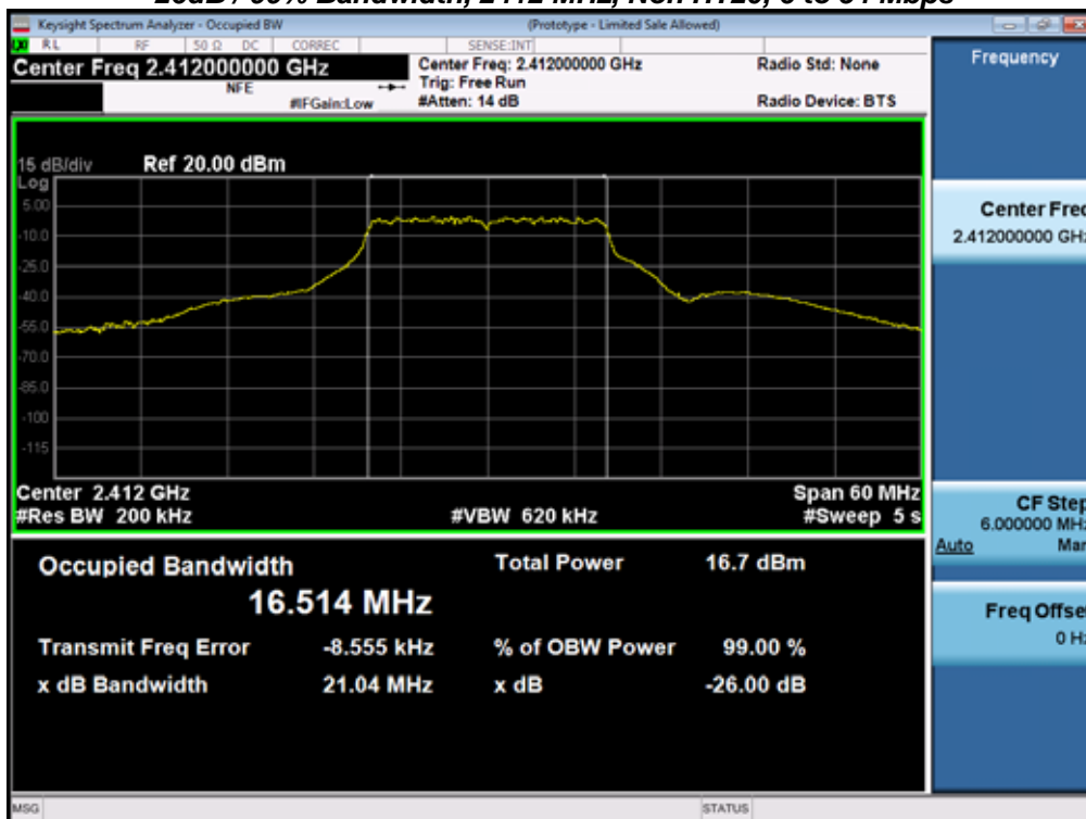
26dB / 99% Bandwidth, 2412 MHz, Non HT20, 6 to 54 Mbps
