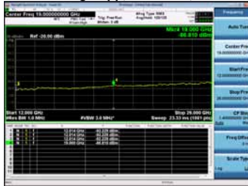
Spurious Of Receive Average Upp, 2412 MHz, Non HT20, 6 to 54 Mbps
