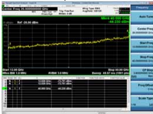
Spurious Of Receive Peak Upper, 5500 MHz, Non HT20, 6 to 54 Mbps
