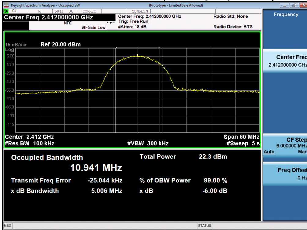
6dB Bandwidth, 2412 MHz, CCK, 1 to 11 Mbps
