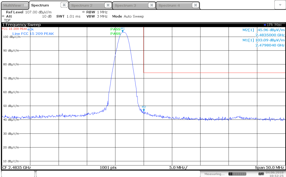
Upper Band Edge, 2480MHz, 8PSK, Peak, (Max: HP)
