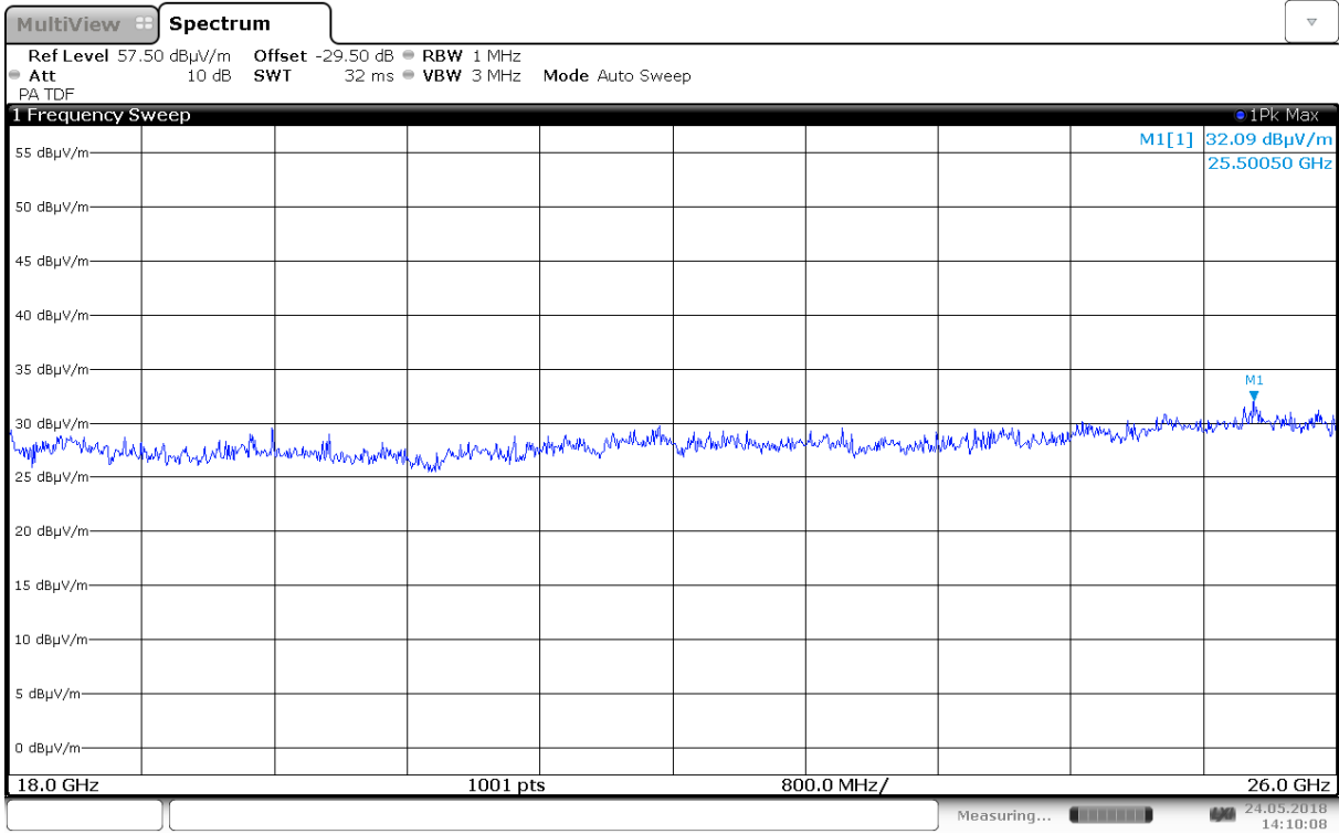
Pre-scan, 18000 -26000MHz, 2440MHz, GFSK, @10cm
