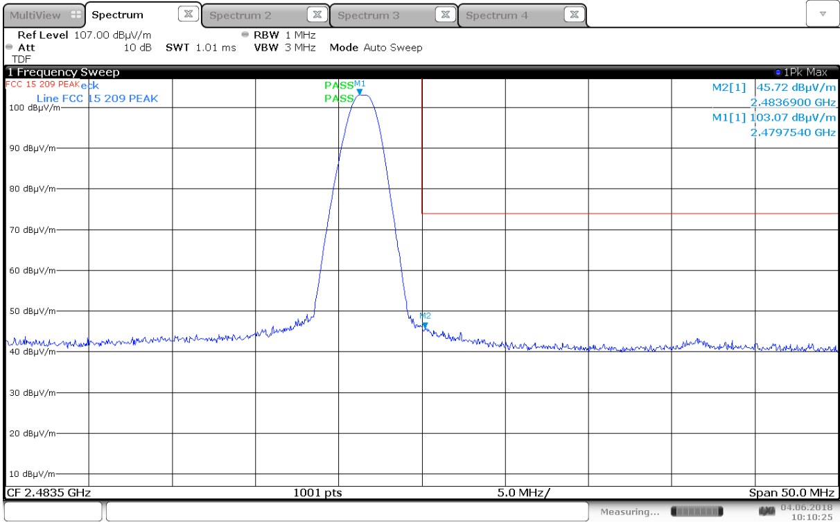
Upper Band Edge, 2480MHz, GFSK, Peak, (Max: HP)
