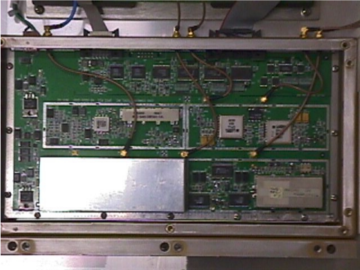
FIG 10. TRANSMITTER OF RF TRANCEIVER
