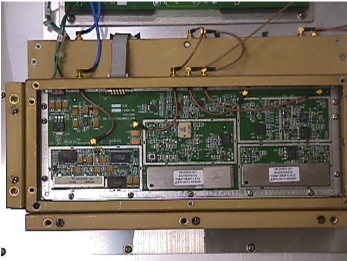
FIG 8. TOP OF RF TRANCEIVER
