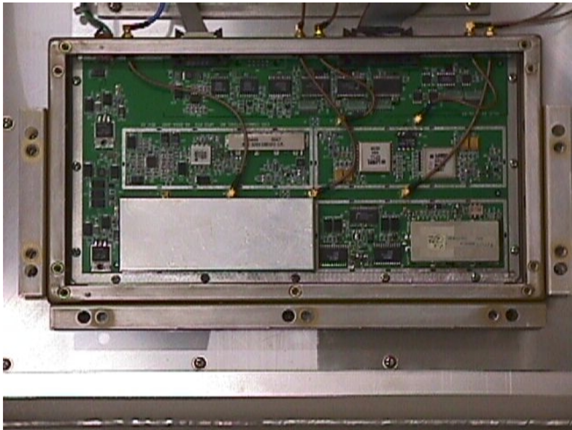
FIG 10. TRANSMITTER(UPCC) OF RF TRANCEIVER
