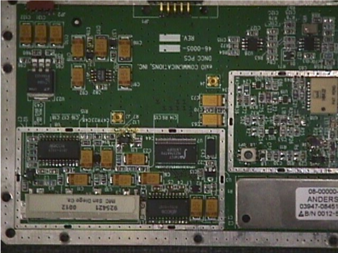
FIG 11. FRONT END OF RECEIVER IN RF TRANCEIVER
