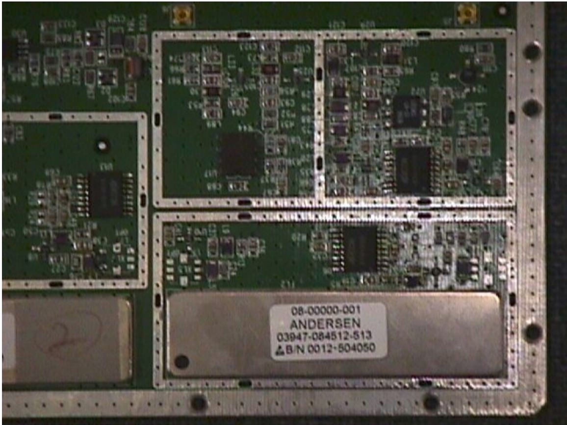
FIG 13. IF BLOCK 2 IN RECEIVER
