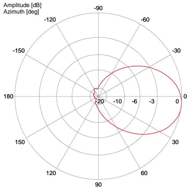
Radiation Pattern
