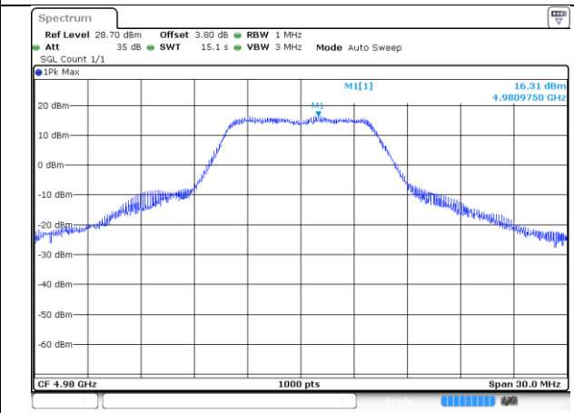
4980-10MHz-802.11a-1-b
