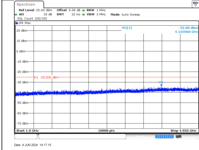
4980-10MHz-802.11a-2-b
