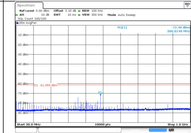
4955-10MHz-802.11n-1-b
