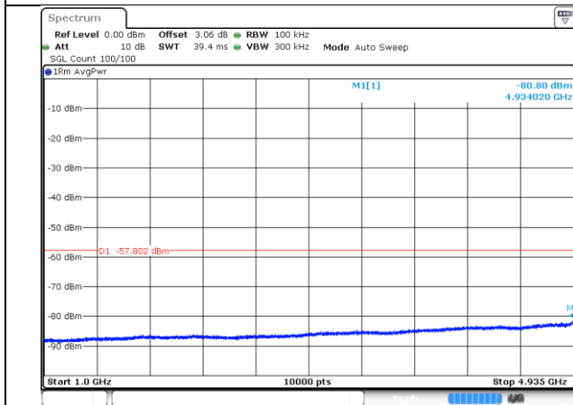
4955-10MHz-802.11n-1-b
