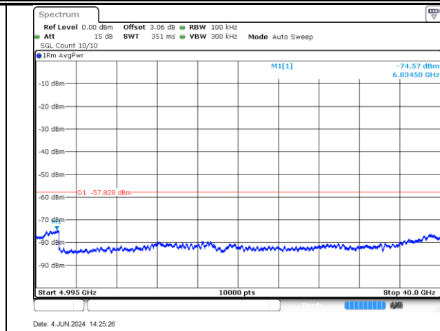
4950-10MHz-802.11n-1-b
